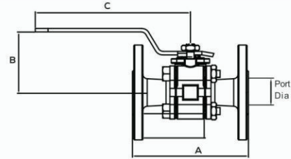
3pc Flanged End Class 150 & Class 300
