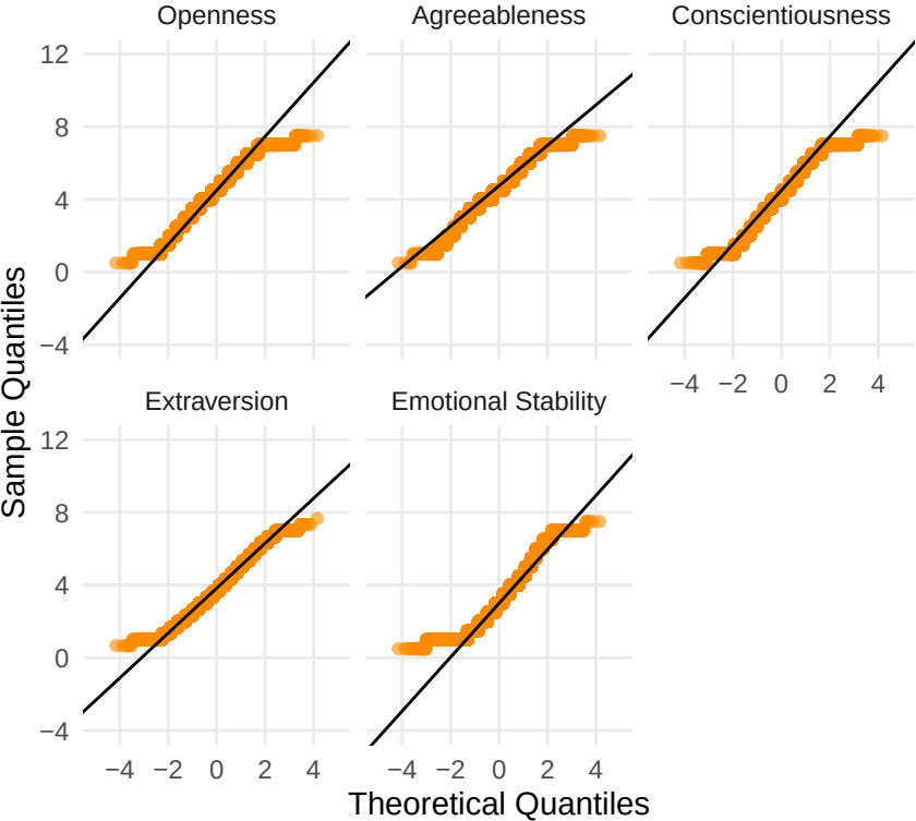
Normal Q-Q Plots for Personality
