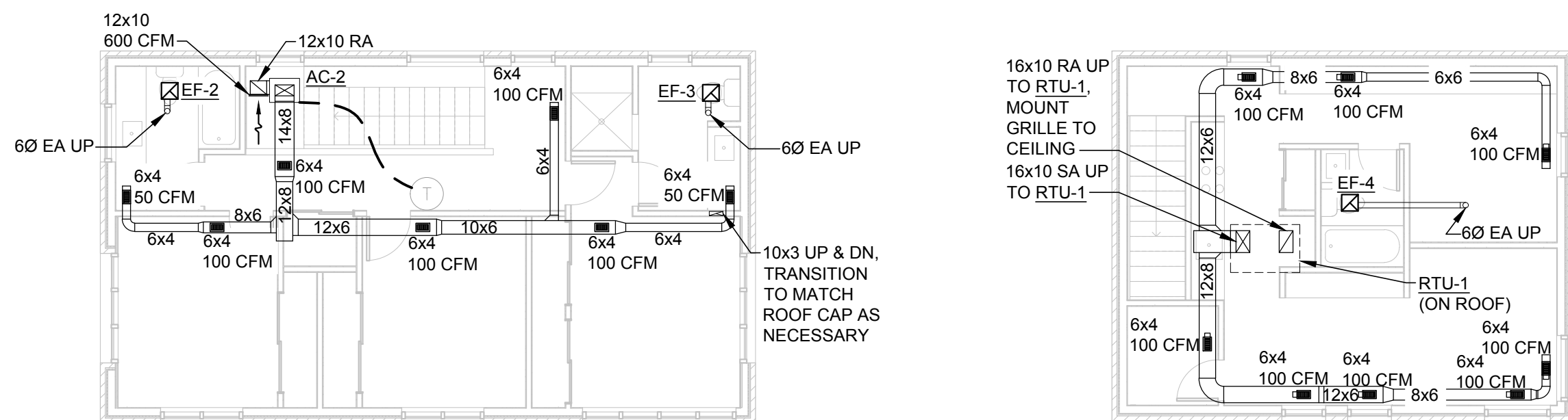
3 SECOND FLOOR HVAC PLAN SCALE: 1/8" = 1'-0"
