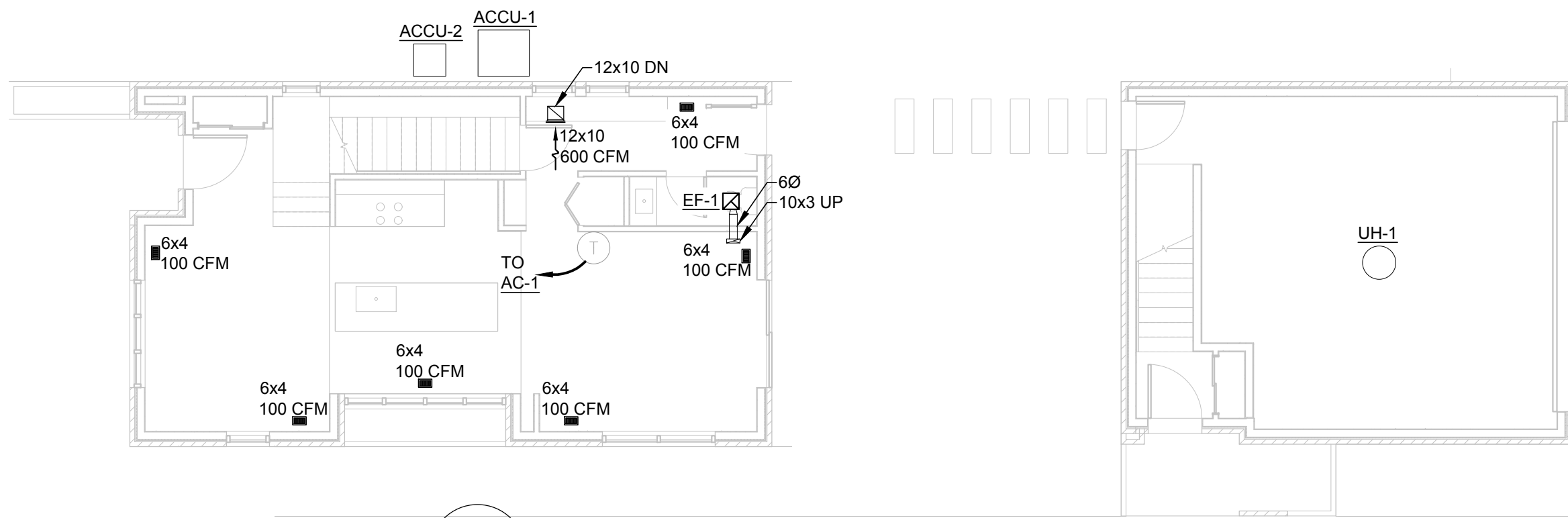
2 FIRST FLOOR HVAC PLAN SCALE: 1/8" = 1'-0"
