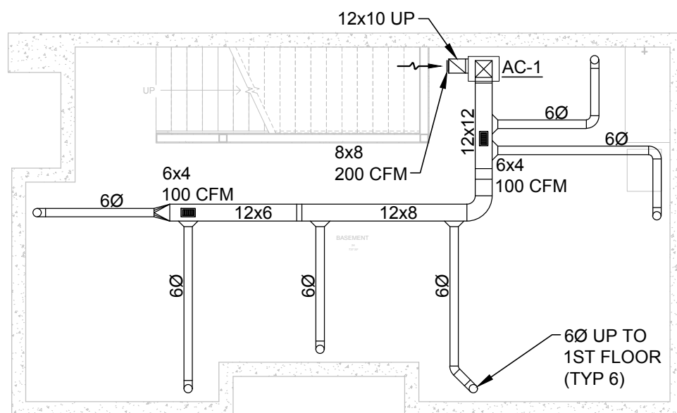
1 BASEMENT HVAC PLAN SCALE: 1/8" = 1'-0"
