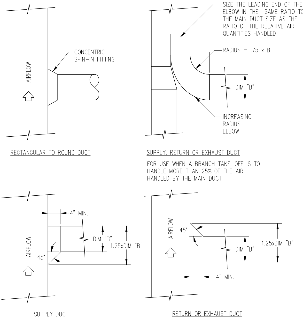
4 RECTANGULAR BRANCH TAKE-OFF DETAILS
