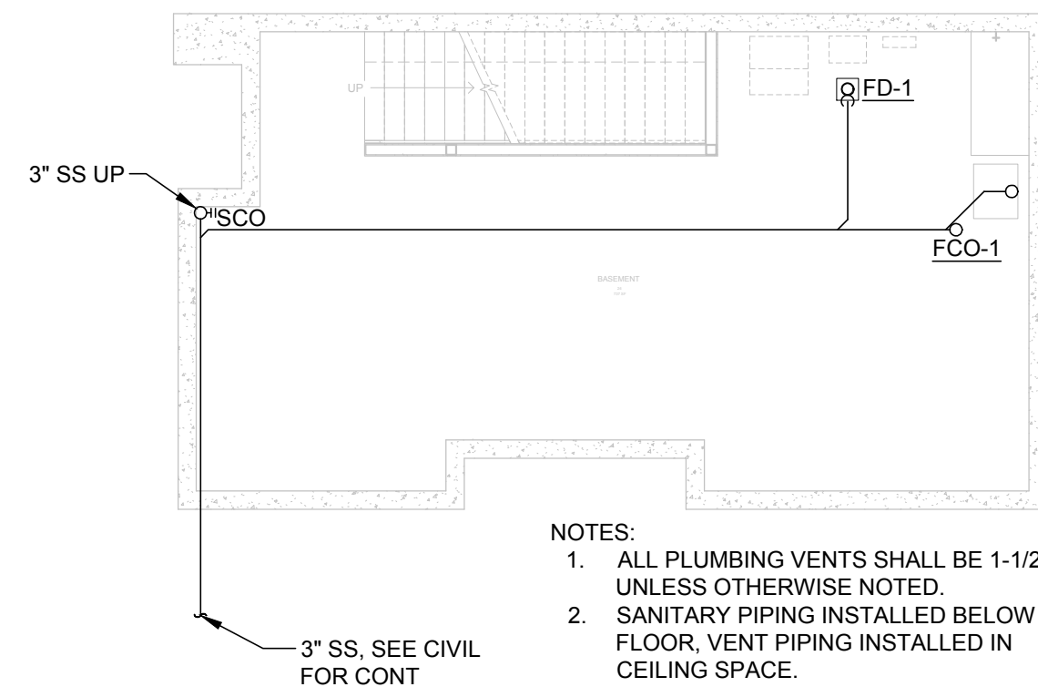
1 BASEMENT WASTE/VENT PLAN SCALE: 1/8" = 1'-0"
