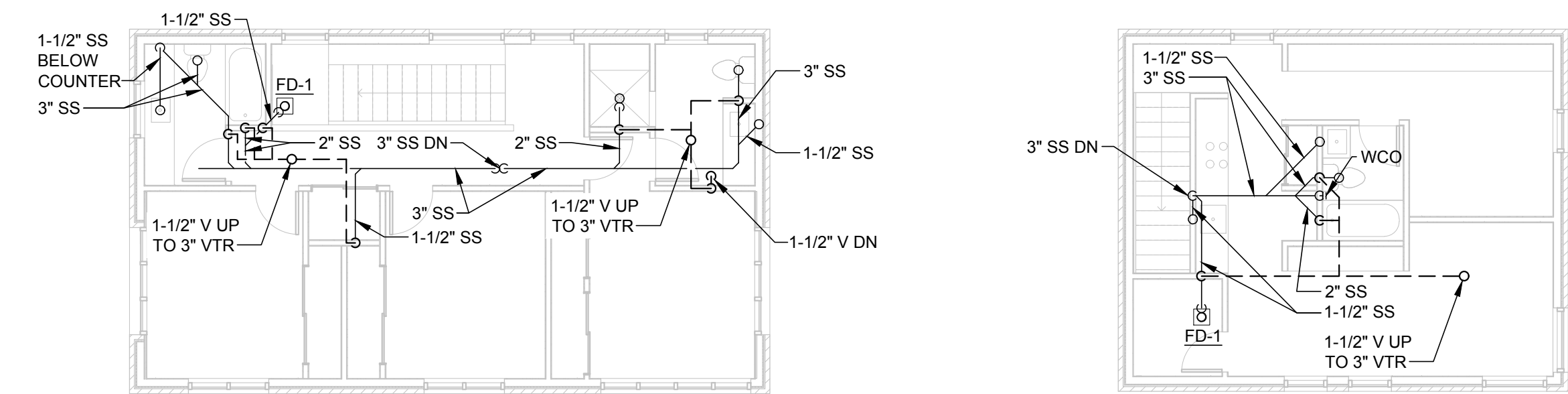
3 SECOND FLOOR WASTE/VENT PLAN SCALE: 1/8" = 1'-0"
