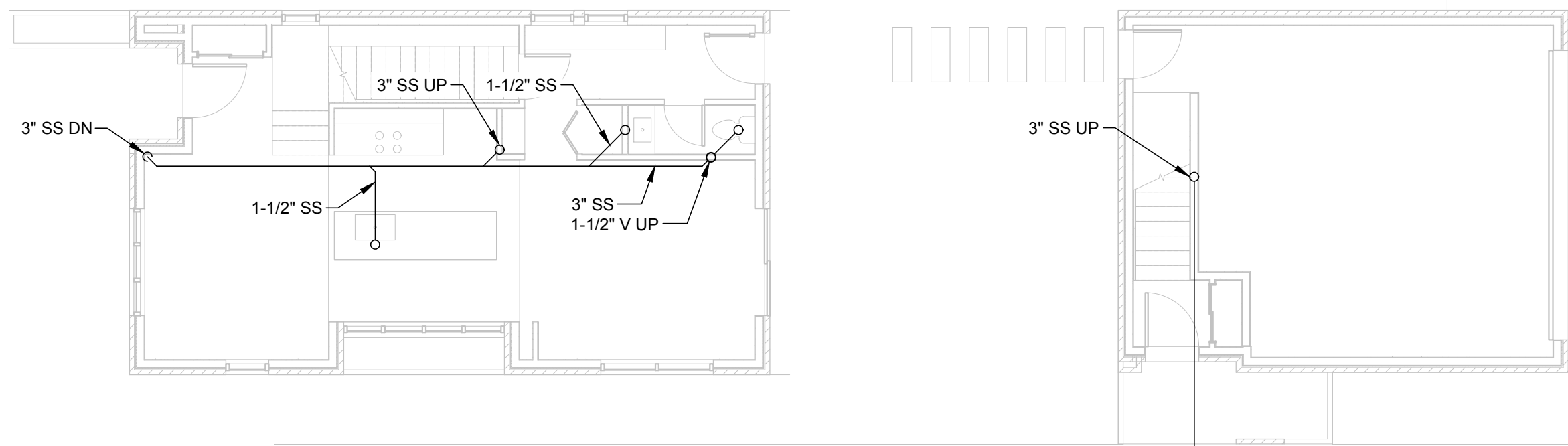
2 FIRST FLOOR WASTE/VENT PLAN SCALE: 1/8" = 1'-0"
