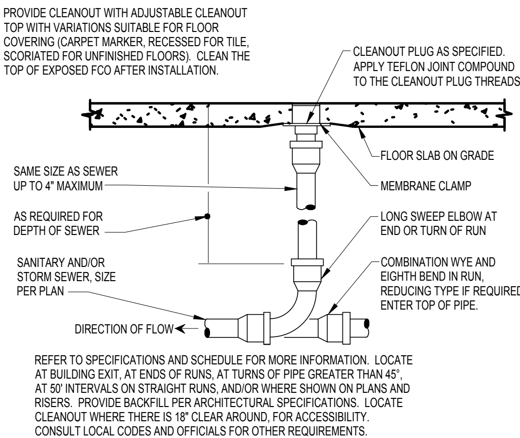
2 FLOOR CLEAN OUT DETAIL Scale: No Scale
