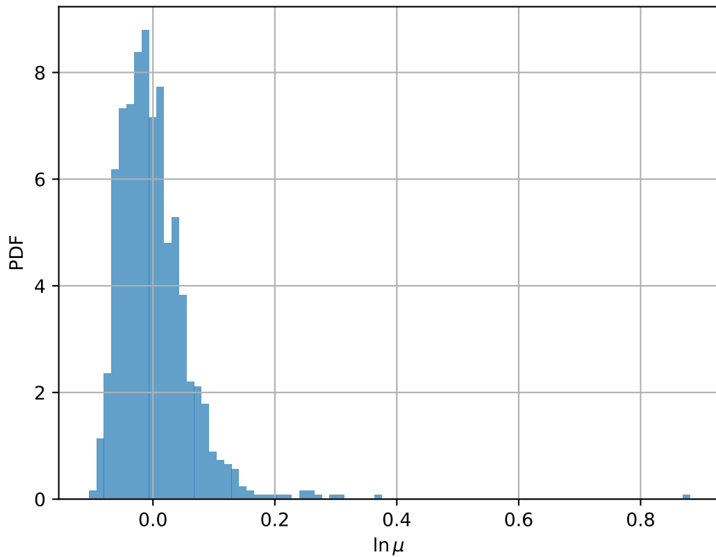
PDF of \ln(\mu)
