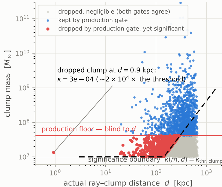
B — matched catalog, ray at r = 300 kpc, f = 10^{-4} : the r -keyed gate discards 61% of this catalog's clump \kappa^2
