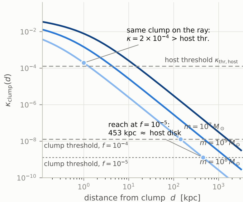
A — one clump: \kappa \propto m/d^2 spans 5 decades, so the threshold must price the worst-case d
