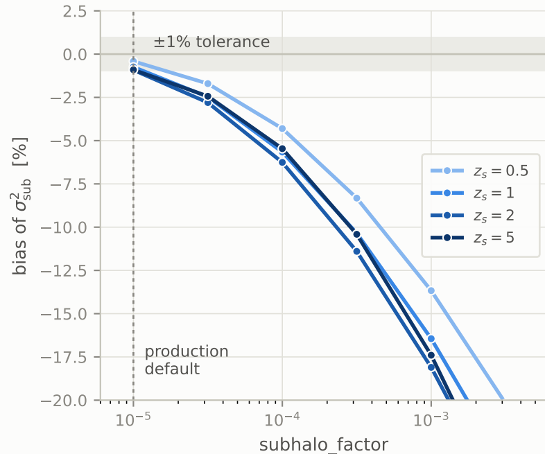
C — the observable: population substructure \kappa -variance bias vs brute force
