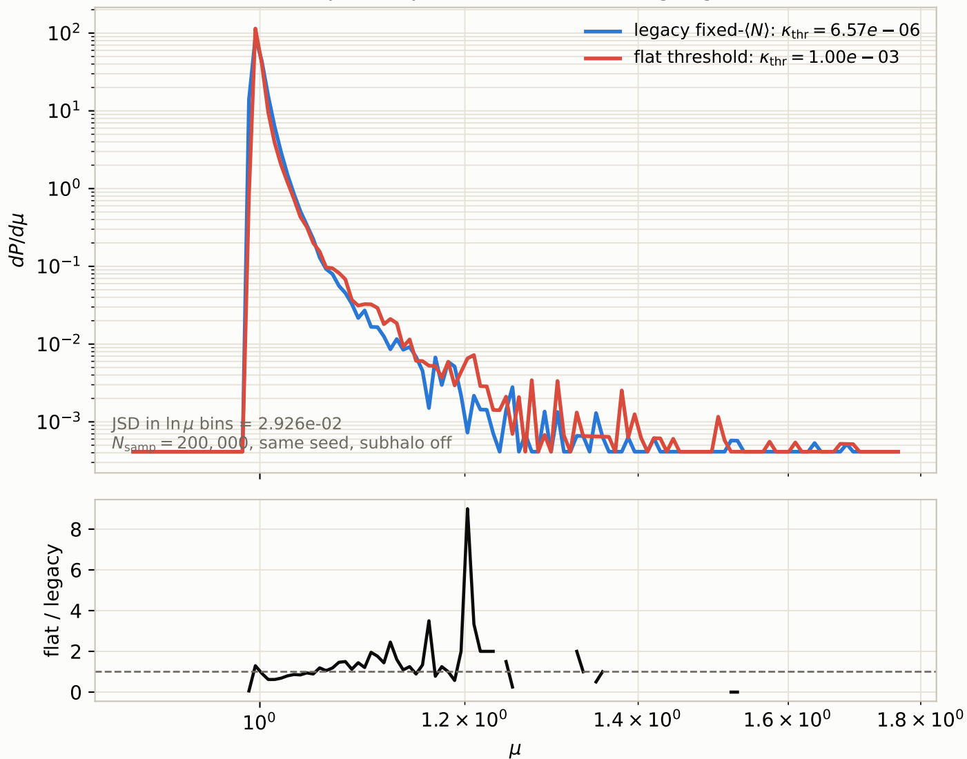
P(\mu) comparison at z_s = 0.2 (log-log)
