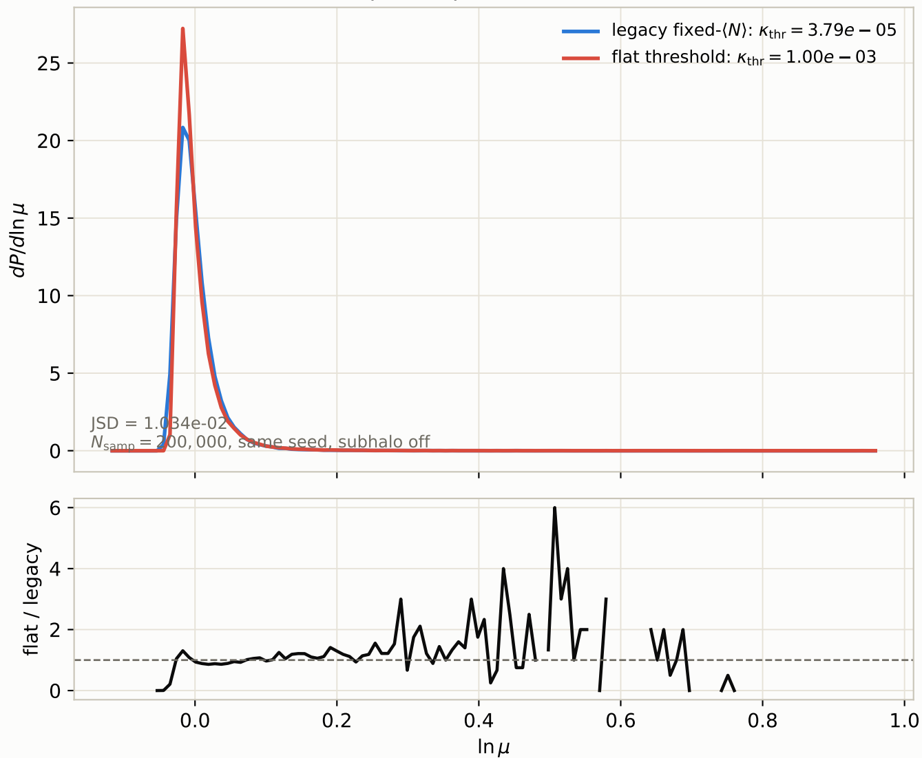
P(\ln \mu) comparison at z_s = 0.5
