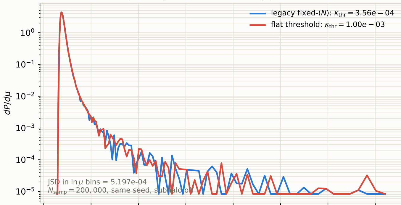
P(\mu) comparison at z_s = 2 (log y, linear x)
