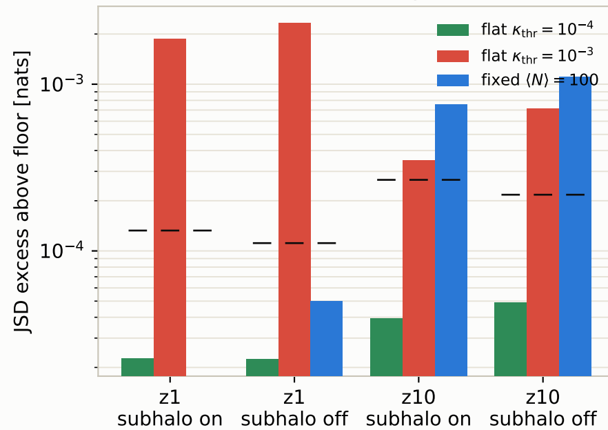
A. Distribution gap to \kappa_{\text{thr}} = 3 \times 10^{-5} truth (dash = finite-sample floor)
