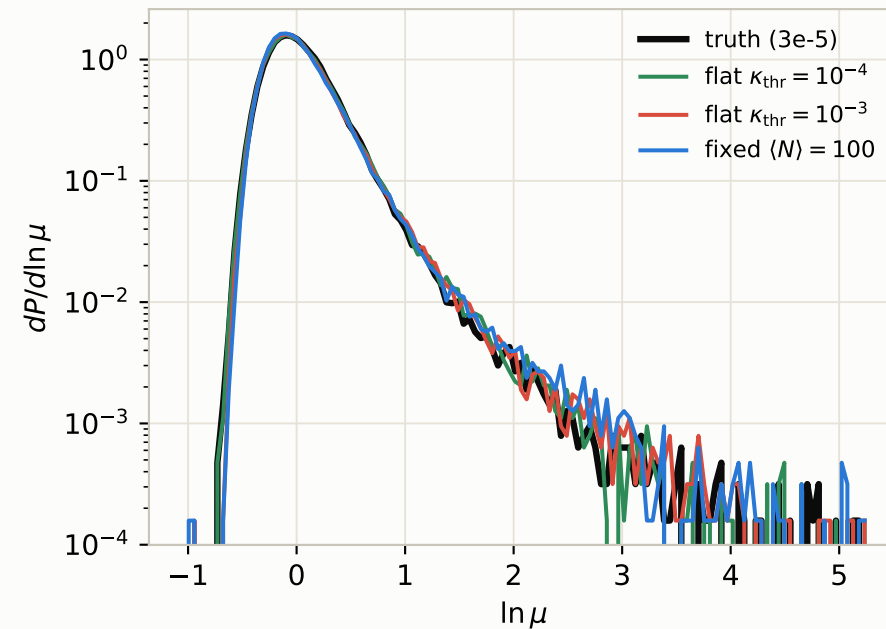
B. z_s = 10 , subhalo ON: P(\ln \mu)
