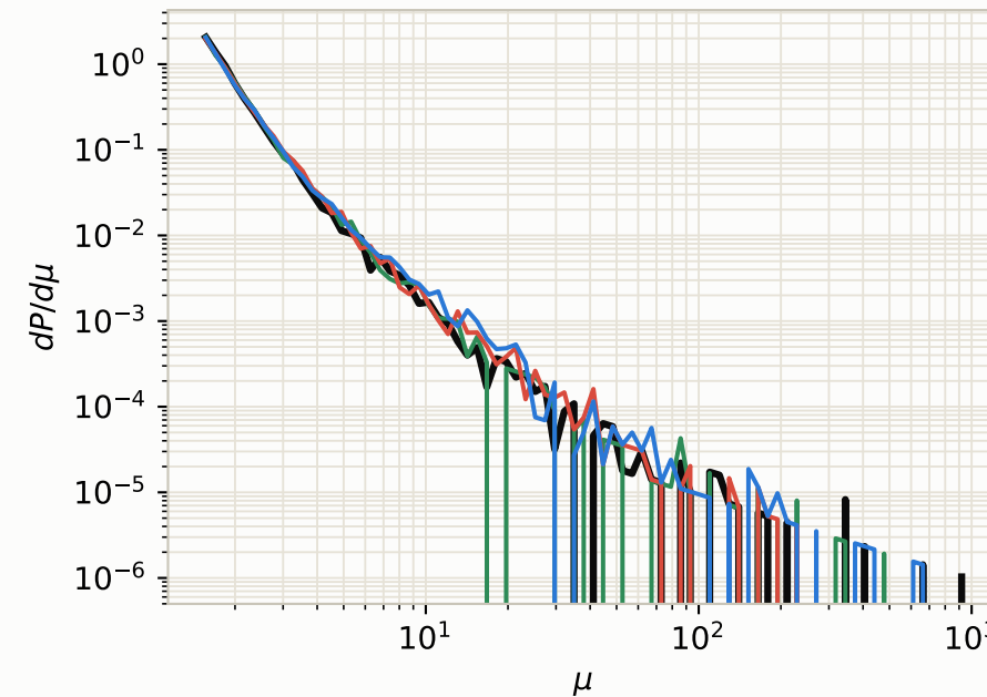
C. z_s = 10 , subhalo ON: magnification tail
