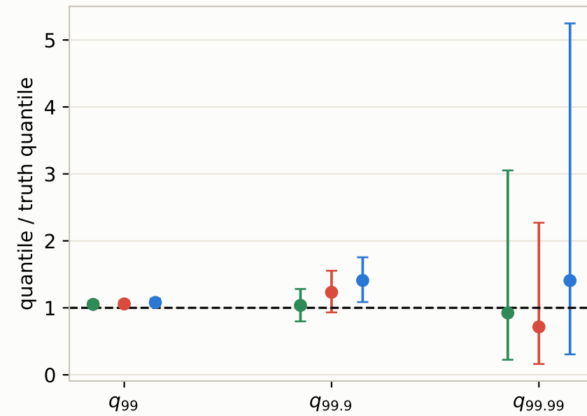
D. z_s = 10 , subhalo ON: tail vs truth (bars = conservative 95% CI)
