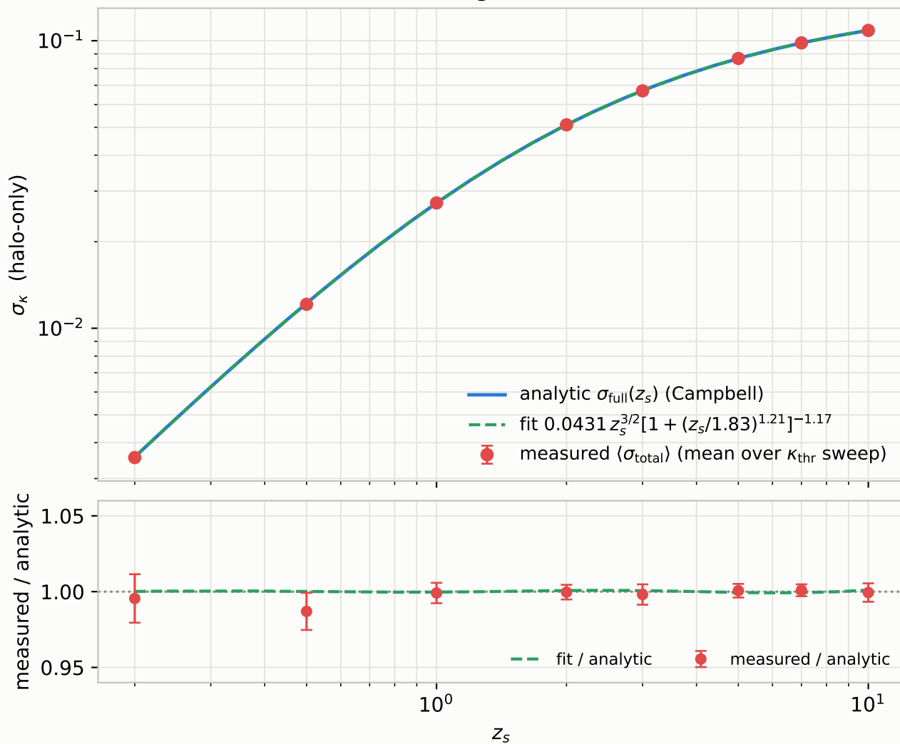
measured total convergence \sigma vs. source redshift
