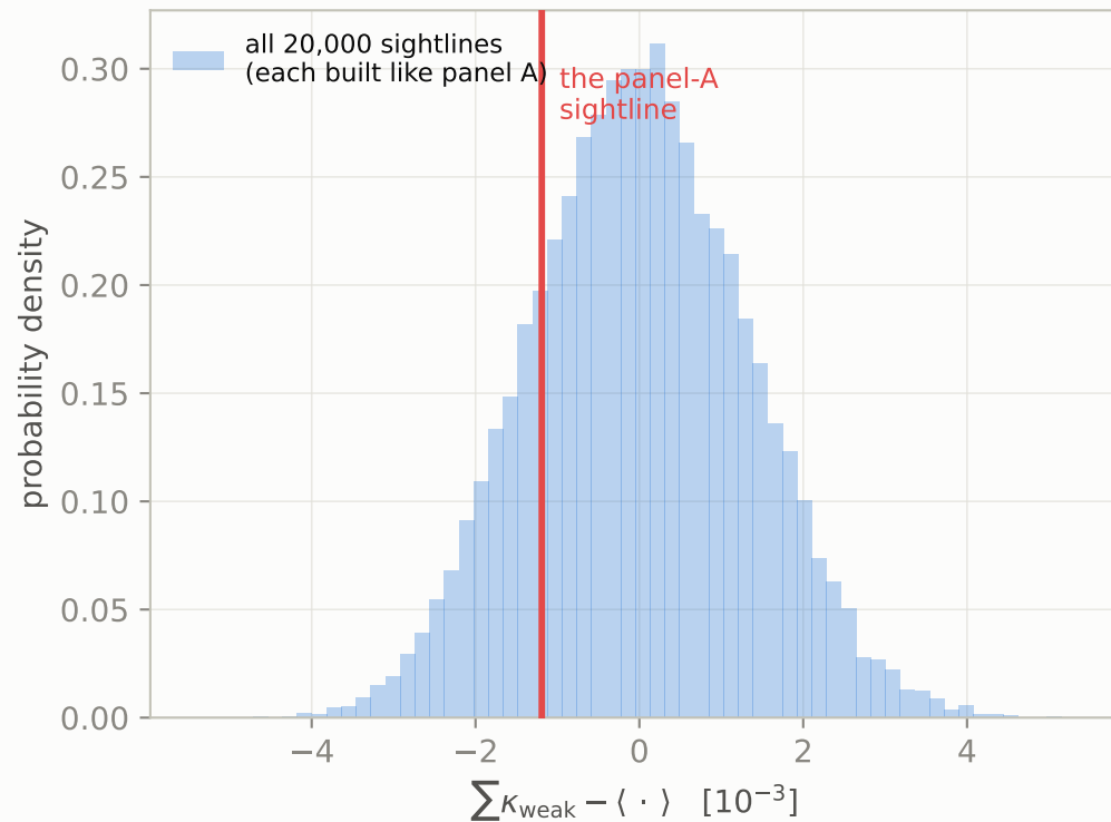
B — that sightline is one draw from the histogram
