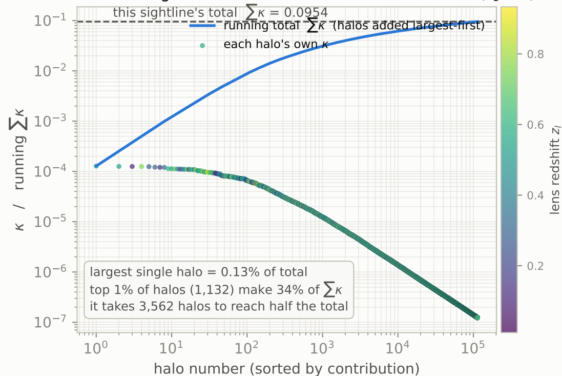
A — one sightline = 113,230 weak halos, summed ( z_s = 1 )
