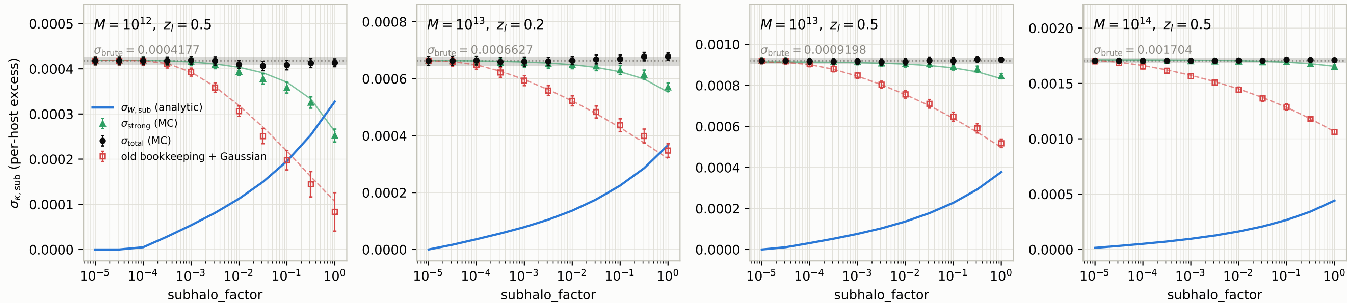
Per-host substructure variance partition, z_s = 1 — strong (resolved-clump MC) \oplus weak (analytic) vs brute
