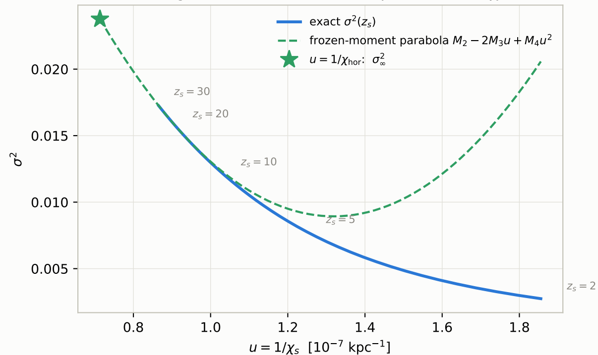
(d) high- z_s closed form: \sigma^2 is a parabola in 1/\chi_s
