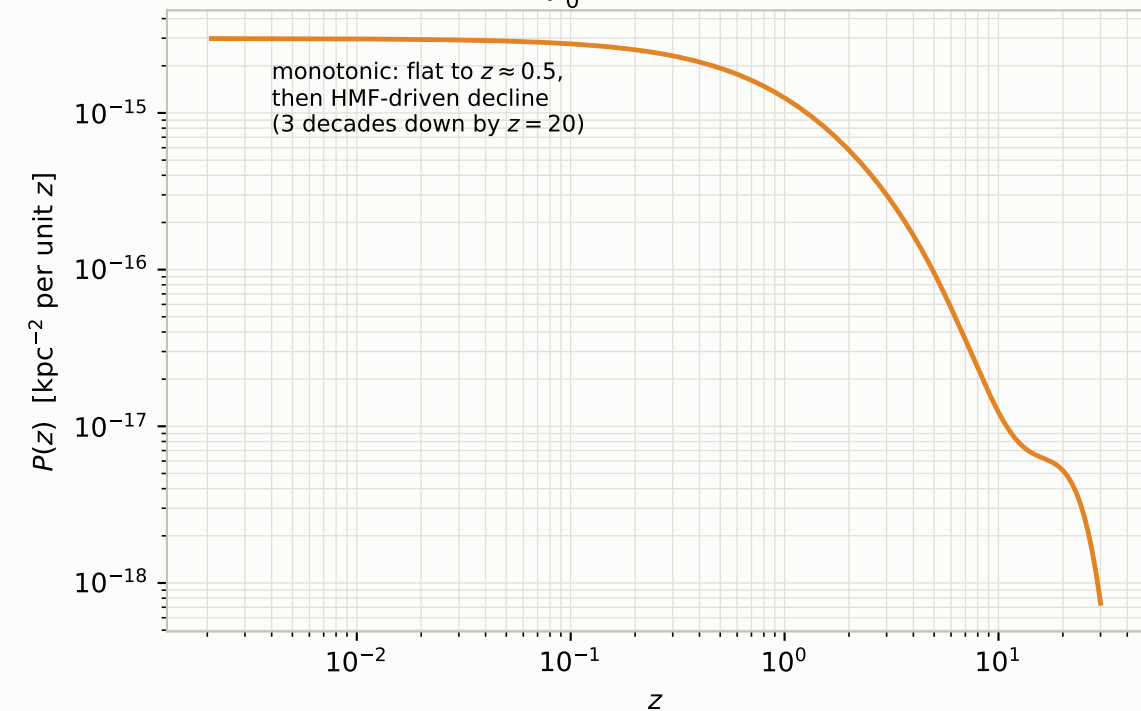
(c) the variance source density P(z)
