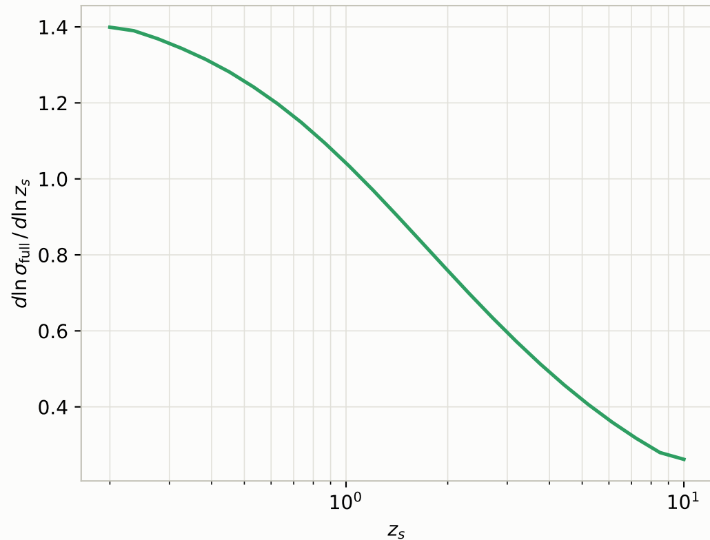
local power-law slope
