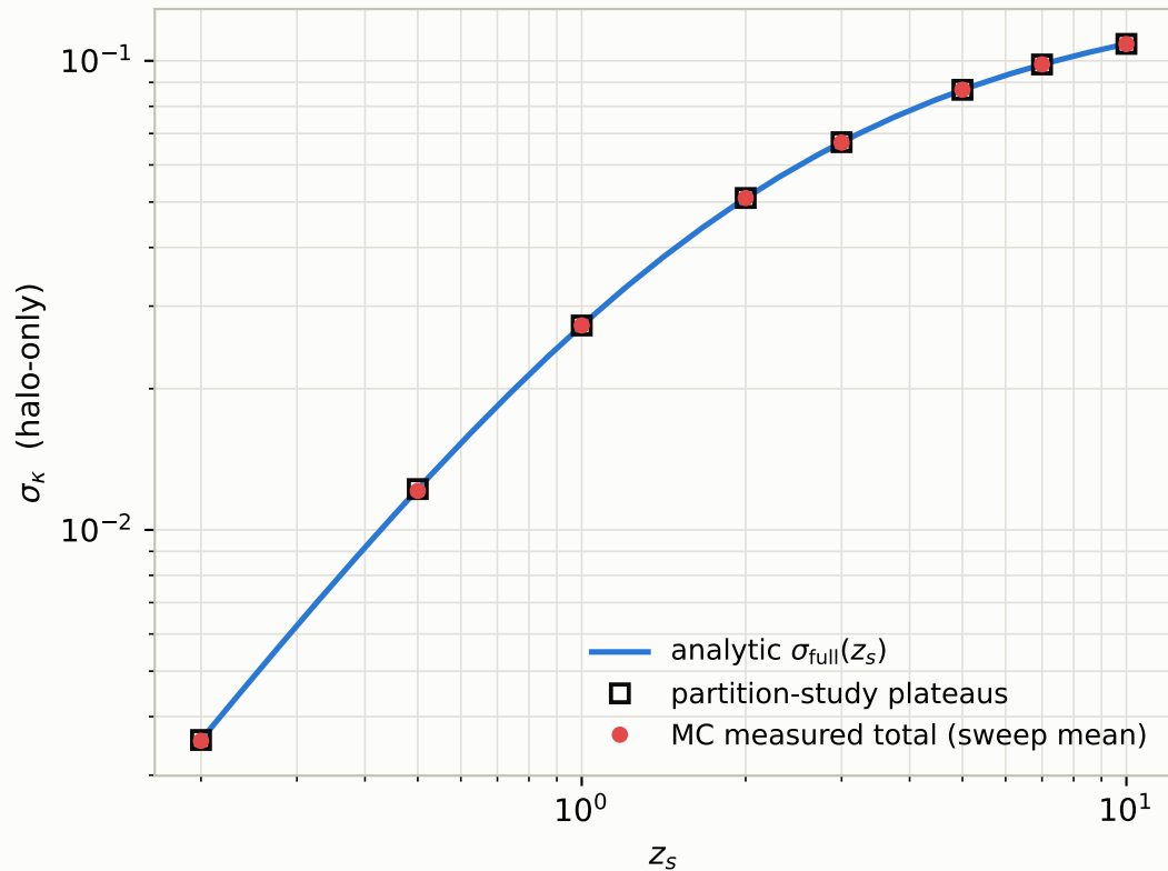
full convergence \sigma vs. source redshift
