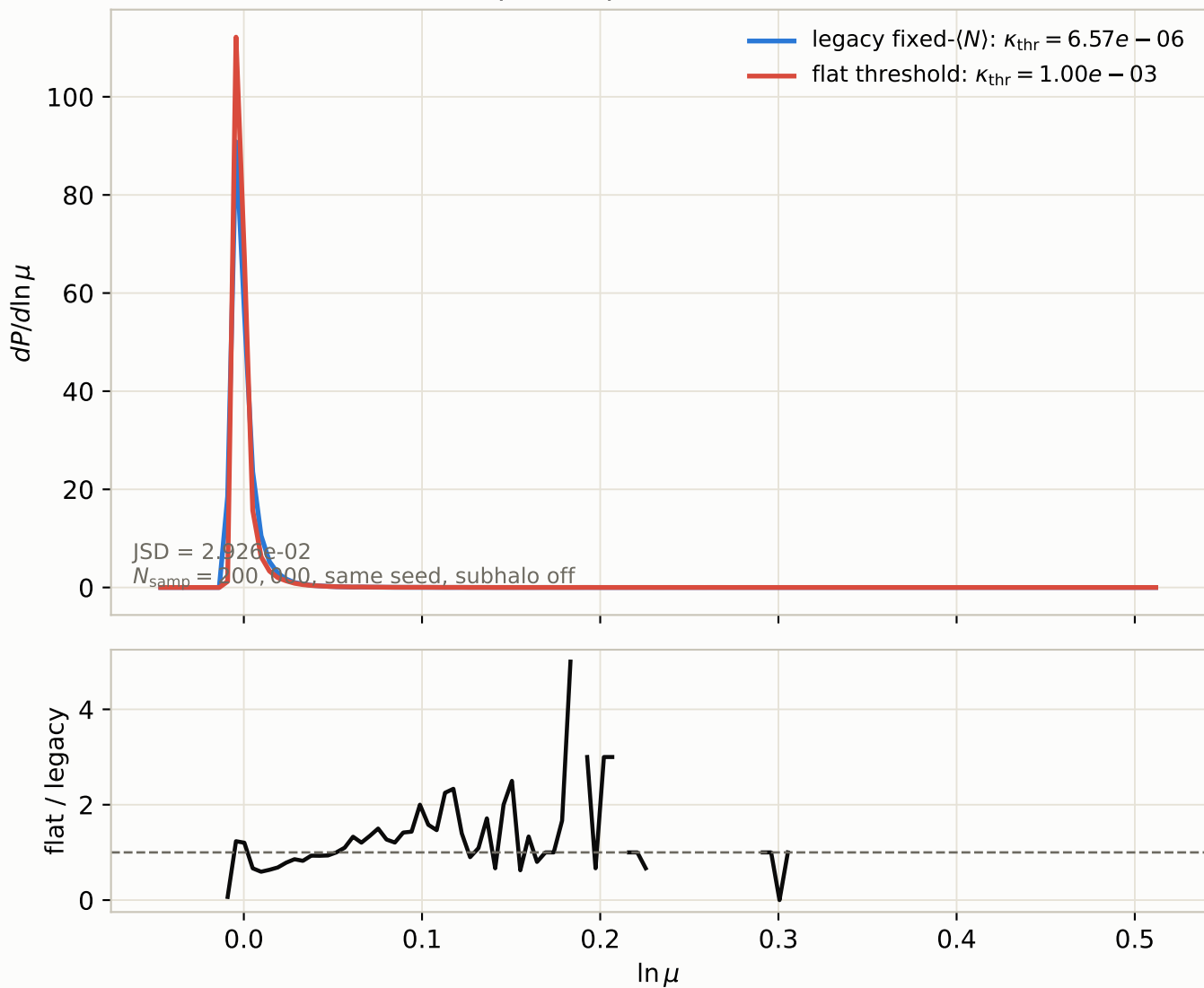
P(\ln \mu) comparison at z_s = 0.2
