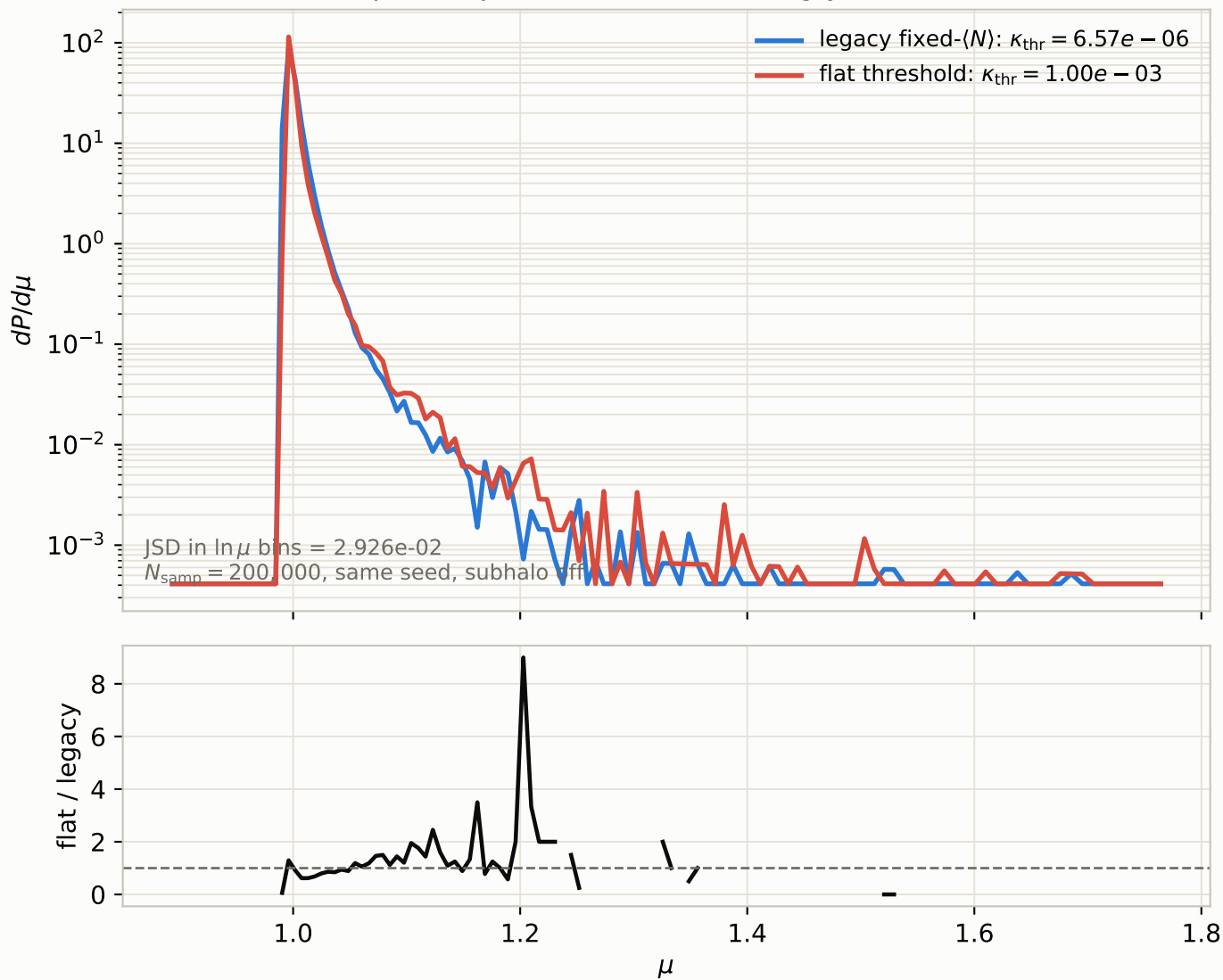
P(\mu) comparison at z_s = 0.2 (log y, linear x)
