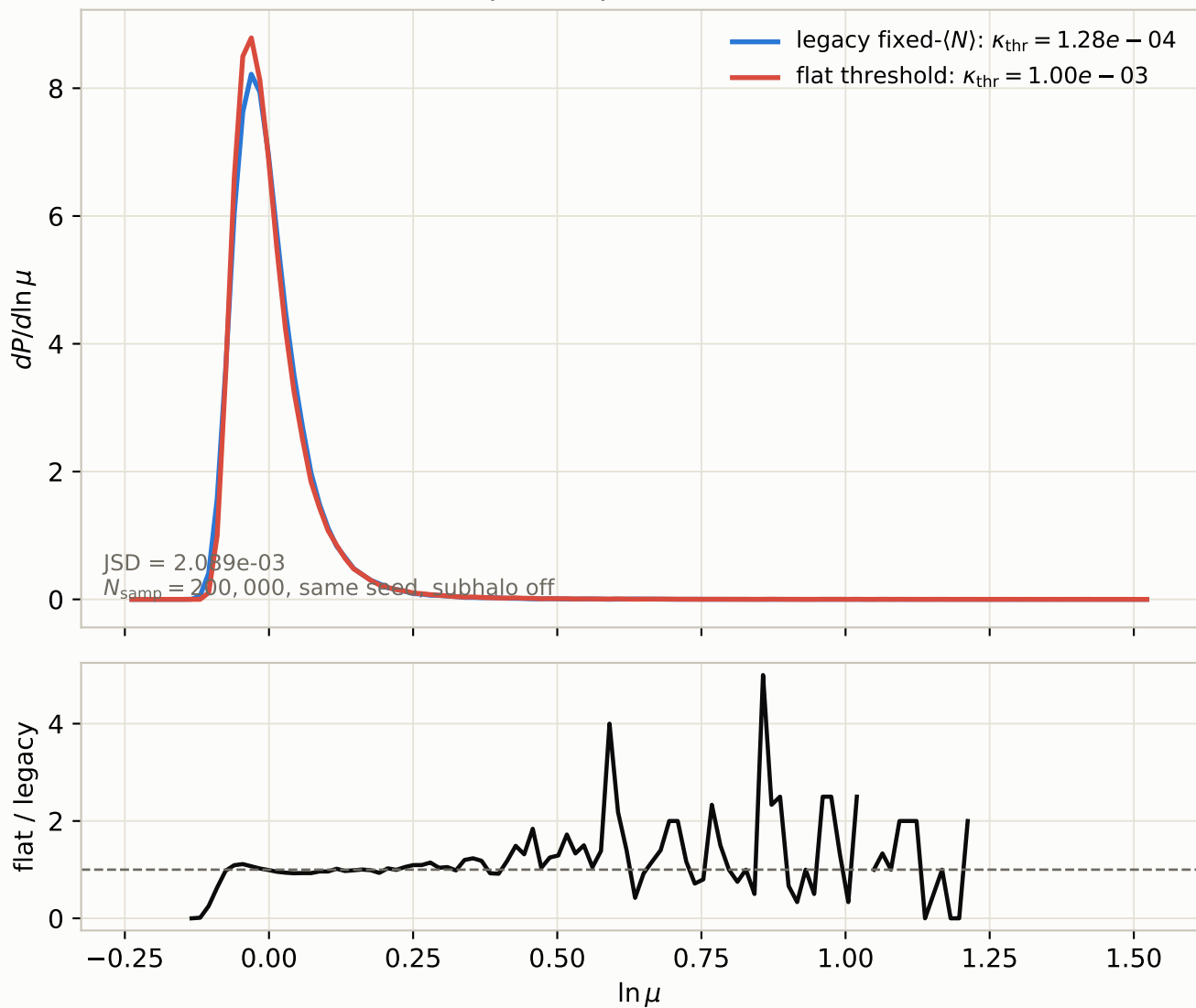
P(\ln \mu) comparison at z_s = 1
