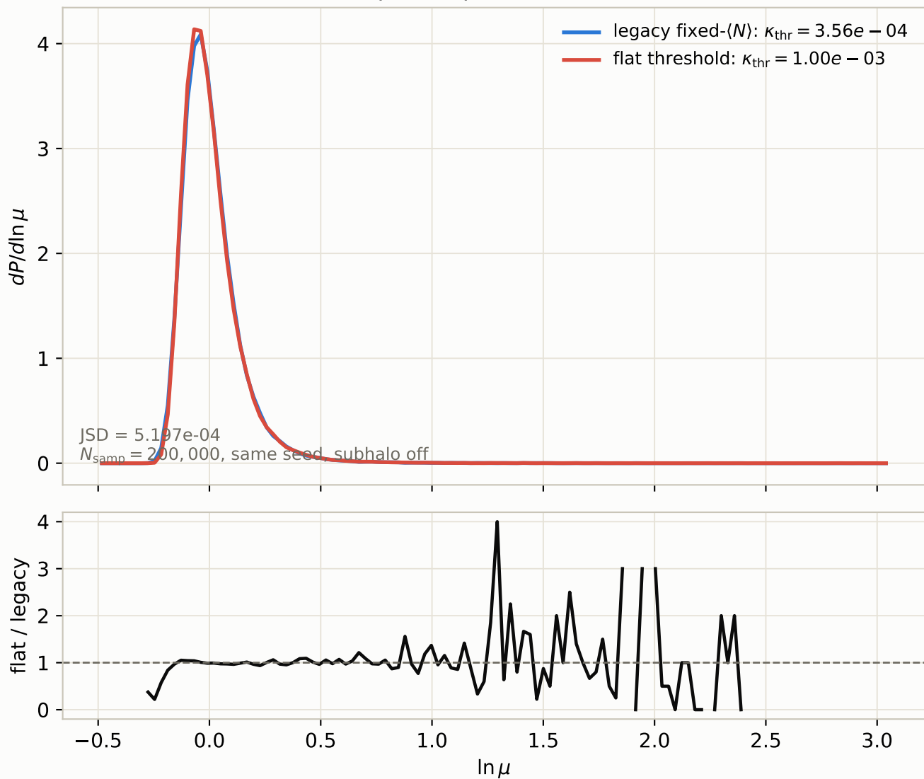
P(\ln \mu) comparison at z_s = 2
