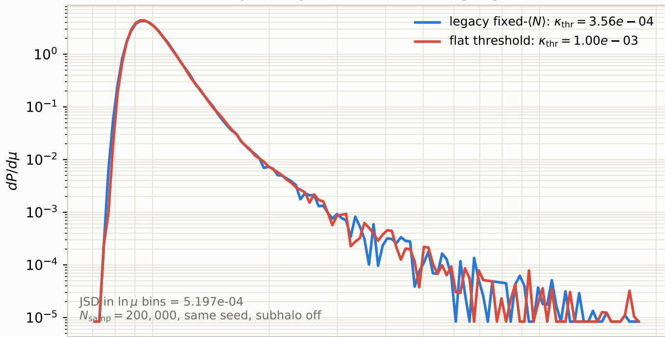
P(\mu) comparison at z_s = 2 (log-log)
