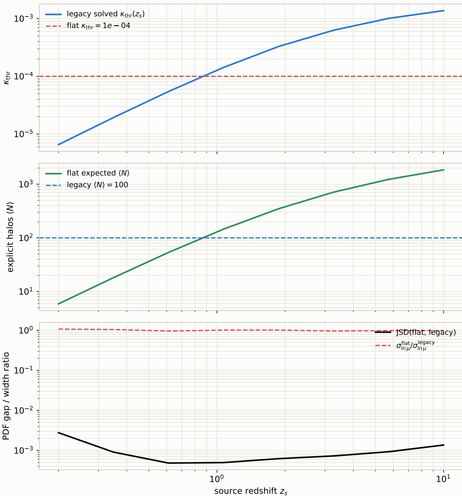
Legacy vs flat-threshold PDF sweep ( \kappa_{\text{thr}} = 1\text{e} - 04 )
