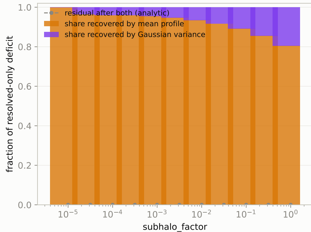
B — what fixes the variance deficit?
