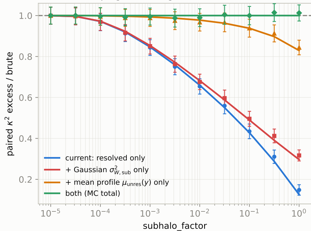
A — bookkeeping closure against brute
