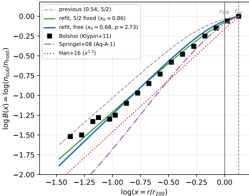
Code units ( r_{200} ), \eta = r_{\text{vir}}/r_{200} = 1.33
