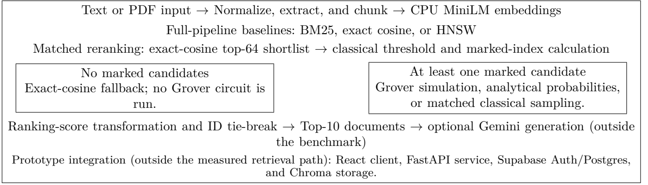
Fig. 3. Prototype architecture and measured retrieval branch. BEIR corpus text is loaded directly; PDF extraction, OCR, and response generation are application context and are not quantitatively evaluated. Matched reranking methods share a classical exact-cosine shortlist, while the reversible score oracle is measured separately as a resource experiment.
