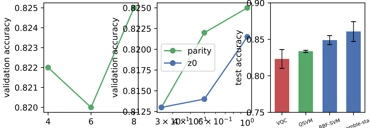
VQC vs circuit width bandwidth and readout quantum vs classical
