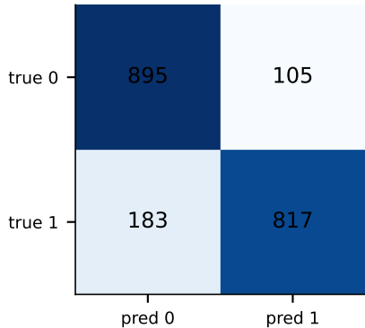
confusion matrix (acc 0.8560)
