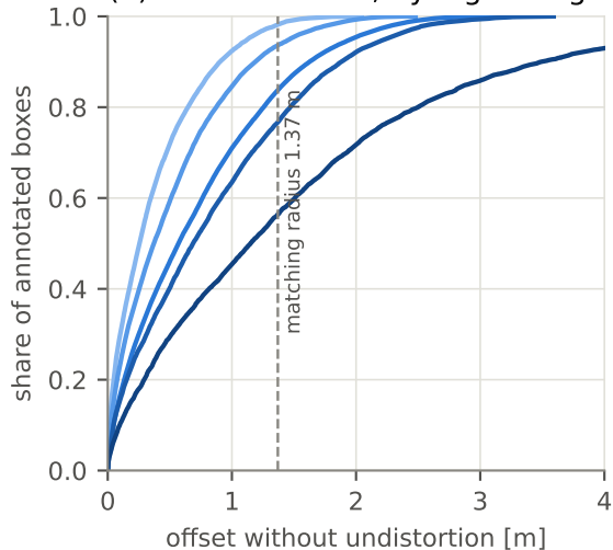
(a) lens distortion, by flight height
