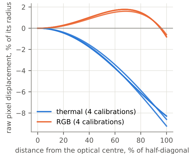
(a) lens distortion of the raw frames (negative: barrel)
