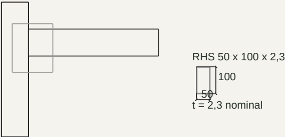
D4 / RAILING-RANGKA
