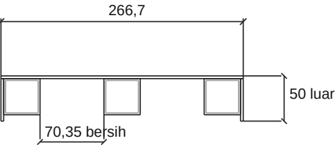
POTONGAN TAPAK / t3 / SHS40x40x2
