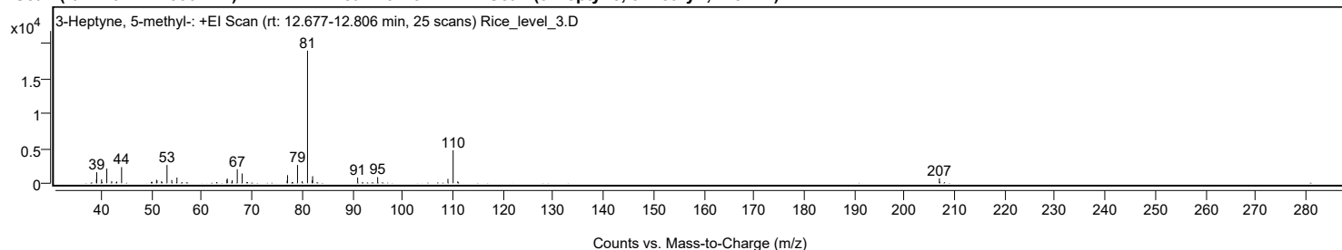
+ Scan (rt: 12.677-12.806 min) Peak 13 from + TIC Scan (3-Heptyne, 5-methyl-, C 8 H 14 )
