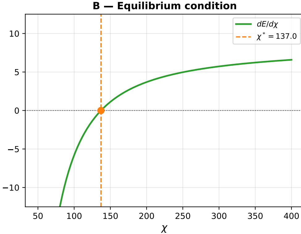
FIG. 2. Equilibrium condition dE/d\chi = 0 . The root is cleanly crossed at \chi = 1/\alpha .
