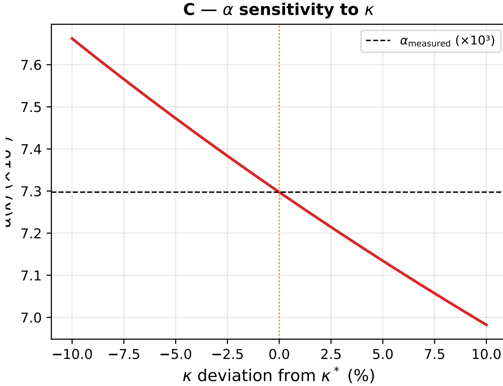
FIG. 3. Sensitivity of the predicted fine-structure constant \alpha to deviations in the underlying transport stiffness \kappa . A 10% variation in \kappa produces only a small fractional shift in \alpha , ensuring stability against macroscopic fluctuations in the medium.
