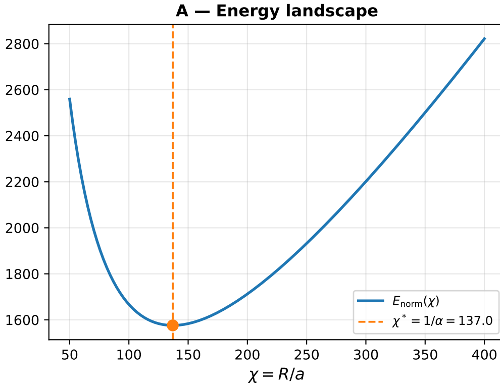
FIG. 1. Energy landscape showing the stable minimum at \chi^* = 137.036 . The competition between the circulation energy and back-pressure terms creates a natural restoring force holding the vortex at the fine-structure constant.
