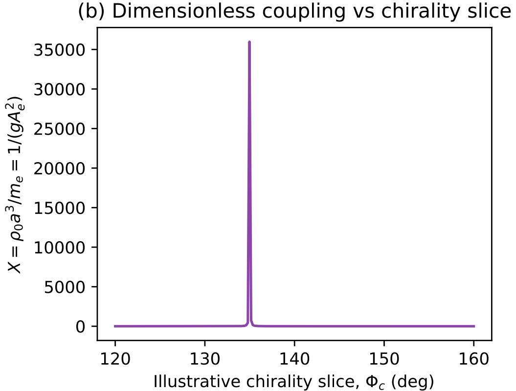
FIG. 2. The dimensionless coupling X computed across an illustrative slice of chirality phase angles \Phi_c . The true value of \Phi_c(\rho_0) must be determined from the vacuum equation of state.
