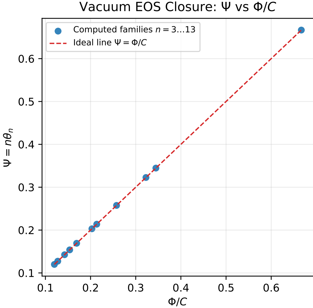
FIG. 2. The equilibrium \Psi_s plotted against \Phi/C across all torus knot families. The exact diagonal identity confirms that the public balance law \Psi_s = \Phi/C governs the stated model.
