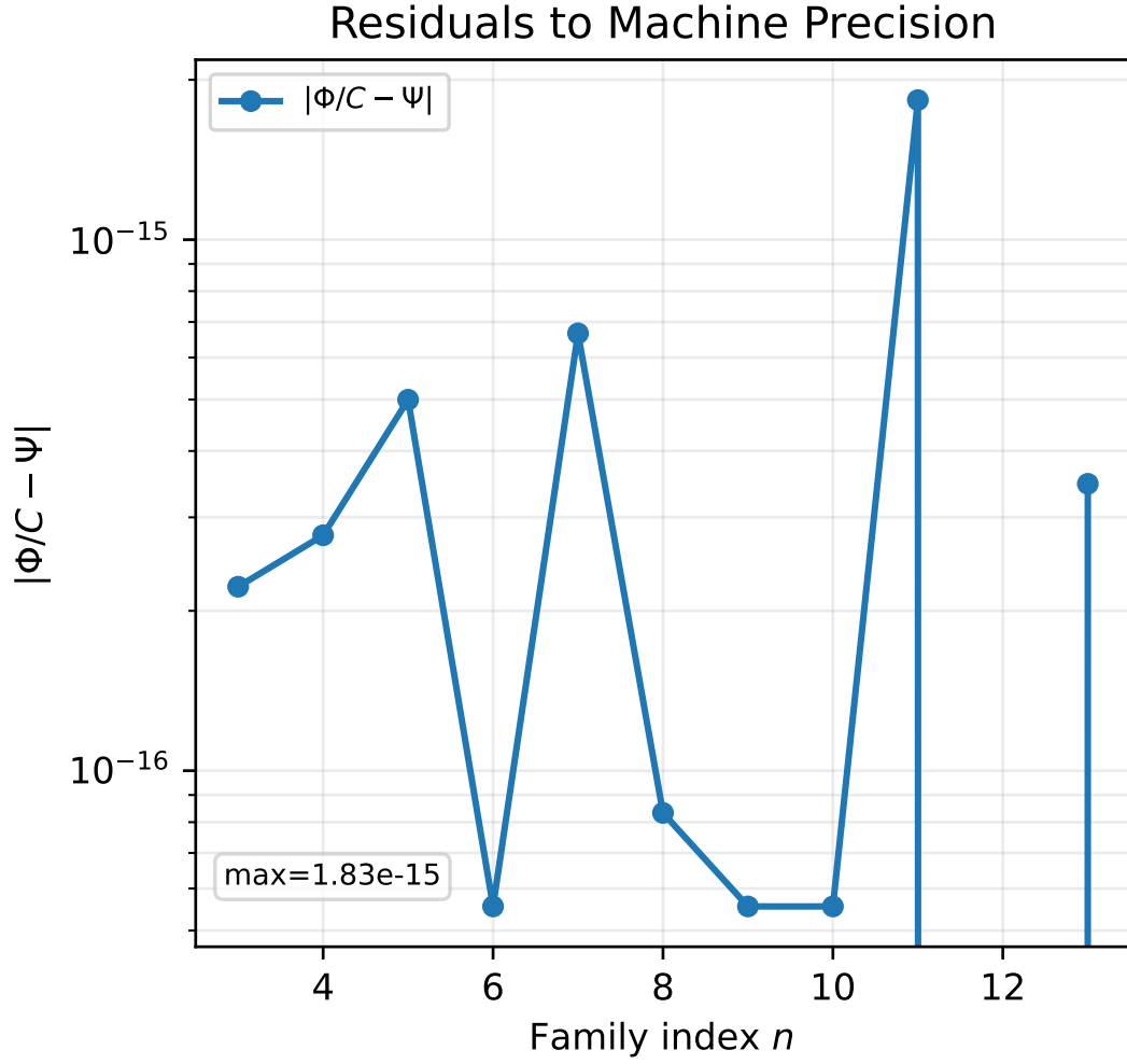
FIG. 3. Absolute residuals |\Phi/C - \Psi_s| . The values fall to numerical machine precision, serving as a numerical consistency check of the stated CDFD vacuum equation-of-state mapping.
