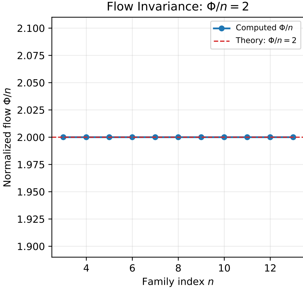
FIG. 1. The flow energy ratio \Phi/n is exactly 2.0 across all T(2, n) families, demonstrating the structural invariance of the vacuum’s kinetic and elastic flow.
