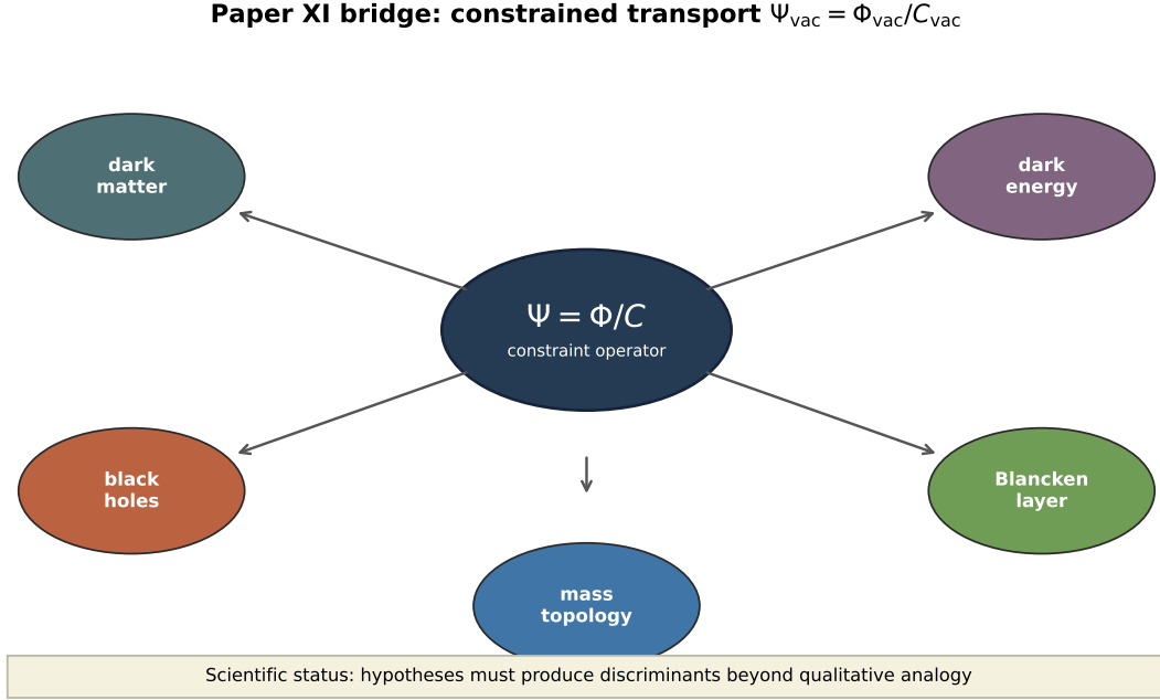
FIG. 1. Cosmological bridge map. Dark matter, dark energy, black-hole saturation, and the Blancken-layer proposal are shown as hypothesis classes attached to the same constrained-transport operator. The lower bar states the required falsification standard.
