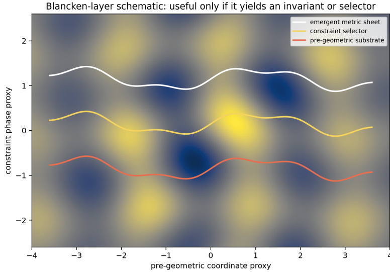
FIG. 7. Reproducible Paper XI conceptual output for the Blancken layer. In the revised manuscript the layer is explicitly marked as speculative until it yields a calculable invariant or boundary condition.
