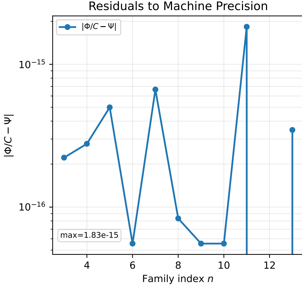
FIG. 5. Archived Paper X residual panel. Residuals near numerical precision support internal consistency of the vacuum equation-of-state calculation; external cosmological validation remains a separate requirement.
