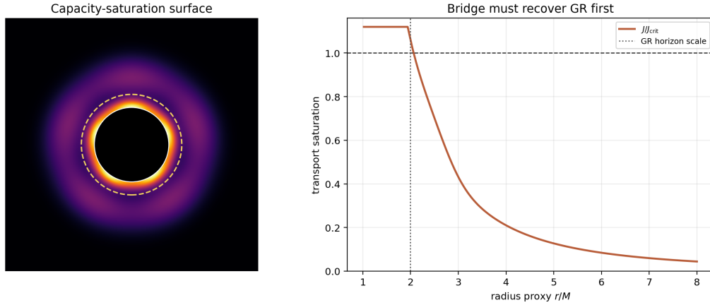
FIG. 6. Reproducible Paper XI conceptual output for black-hole rupture. The figure is retained as a transport-capacity visualization; the actual physics claim must be tested through horizon, ringdown, or thermodynamic discriminants.
