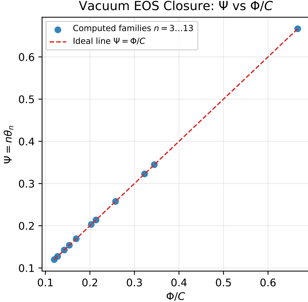
FIG. 4. Archived Paper X vacuum equation-of-state check: the equilibrium variable \Psi_s tracks \Phi/C across the torus-knot family. In this synthesis paper the same relation is used only as a bridge assumption for cosmological hypotheses, not as direct evidence for the dark sector.
