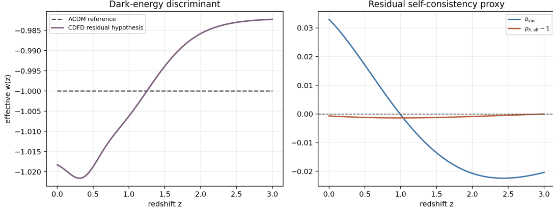
FIG. 3. Reproducible Paper XI conceptual output for adaptive expansion. The revised claim is narrower: cosmic acceleration is modeled as a residual of incomplete vacuum self-consistency, not as proof that the residual has already been derived from first principles.
