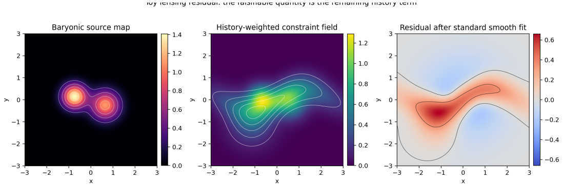
FIG. 2. Reproducible Paper XI conceptual output for the dark-matter claim: persistent flux aggregation hardens the surrounding constraint geometry, producing lensing-like curvature. In this manuscript the image is treated as a conceptual model, not as observational evidence.
