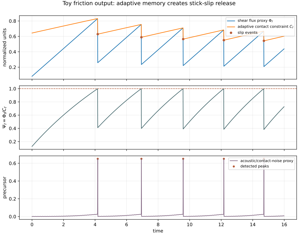
FIG. 2. Generated stick-slip output. A slowly increasing shear-flux proxy loads an adaptive contact constraint until release. The lower panel shows a precursor/noise proxy. Event table: table2_friction_stick_slip_events.csv .
