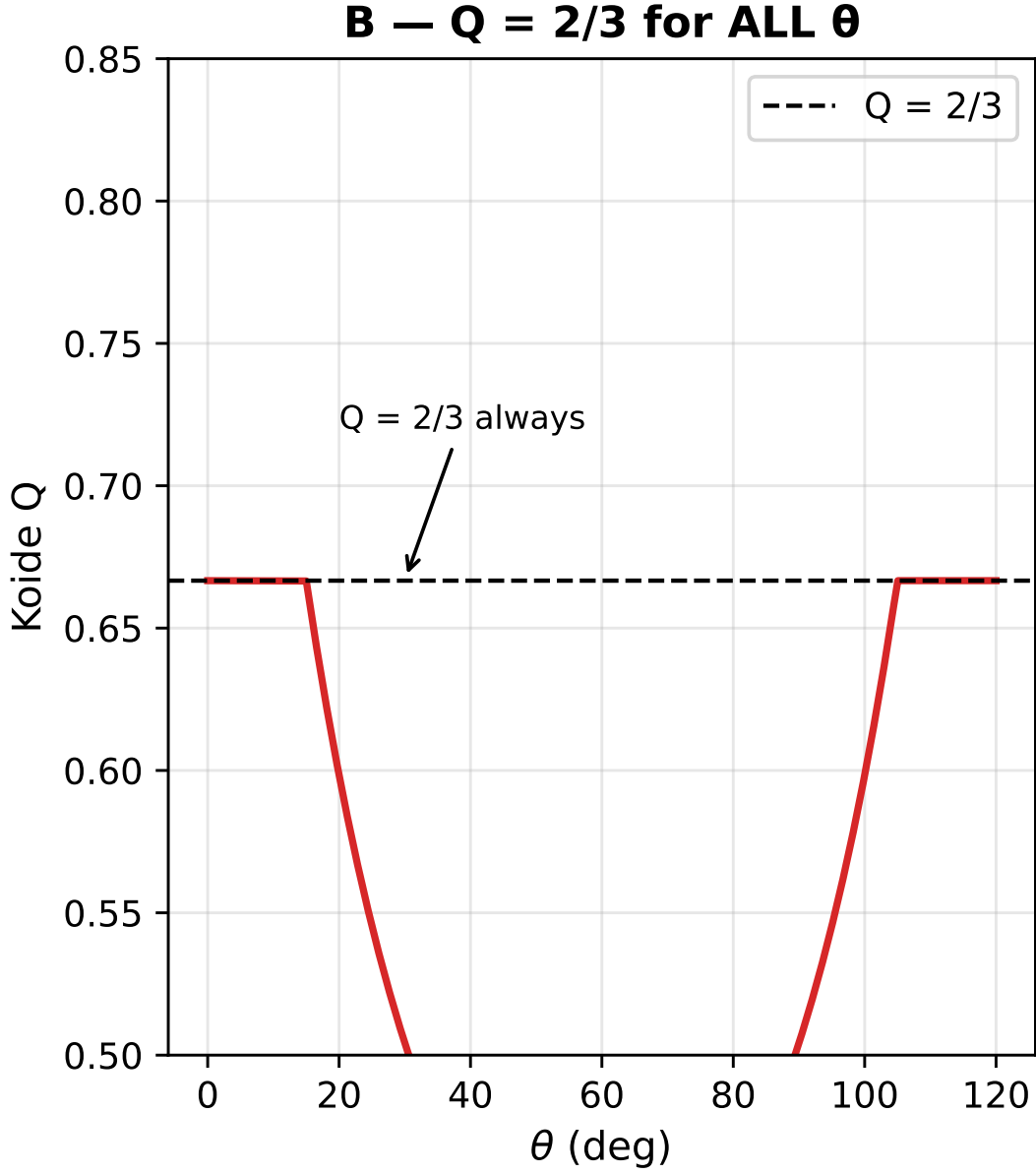
FIG. 3. The Koide ratio Q evaluates to exactly 2/3 for all possible values of \theta , demonstrating that the formula is a direct consequence of the \mathbb{Z}_3 symmetry rather than a parameter-tuned coincidence.
