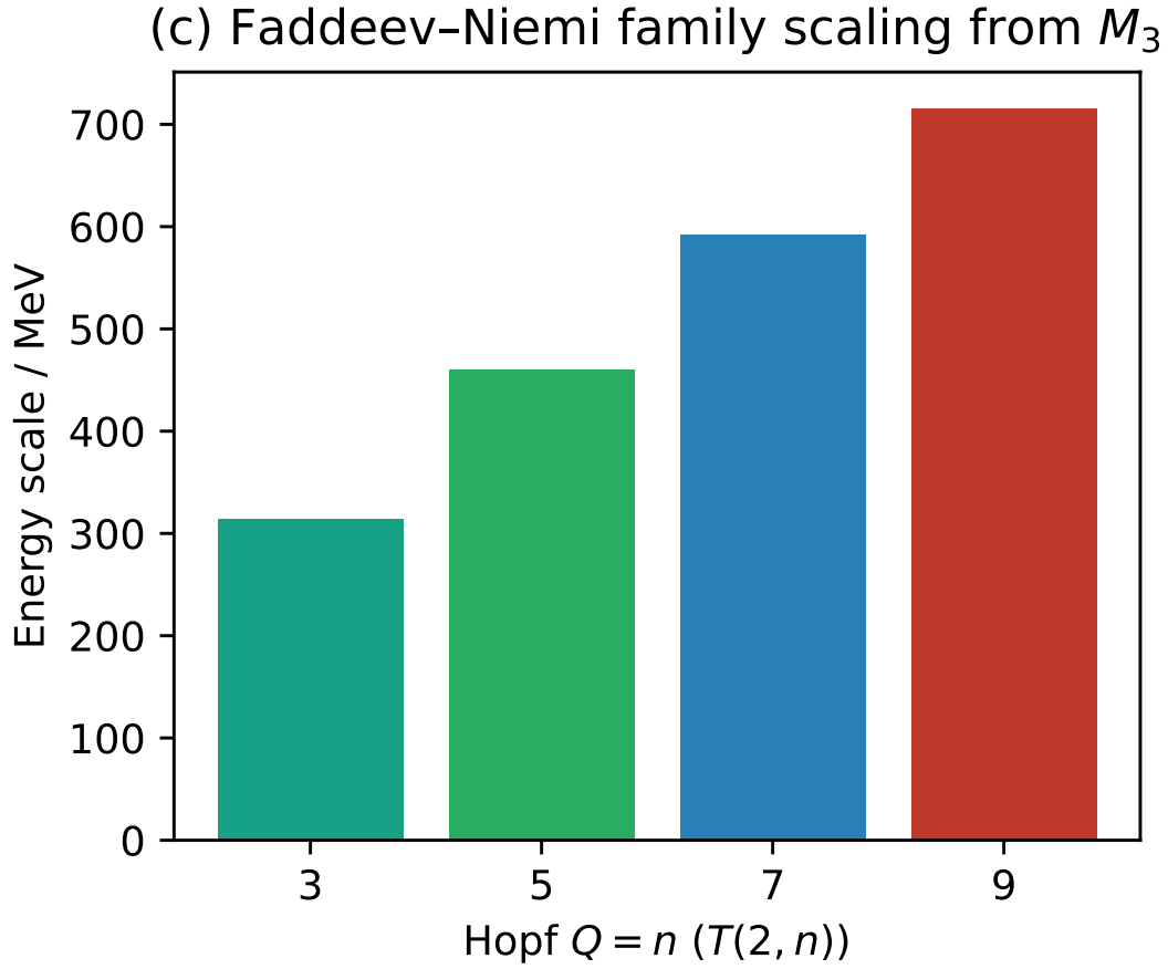
FIG. 3. Faddeev–Niemi family scaling predicting the energy scales of higher knotted soliton families (cinquefoil n = 5 , etc.) directly from the lepton trefoil scale M_3 \approx 313.9 MeV.
