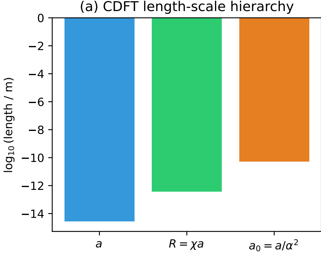
FIG. 1. The CDFT length-scale hierarchy. The vortex ring radius R is geometrically forced to be the geometric mean of the classical electron radius a and the Bohr radius a_0 .
