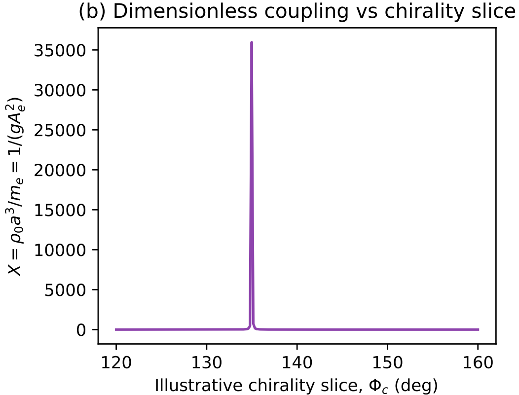
FIG. 2. The dimensionless coupling X computed across an illustrative slice of chirality phase angles \Phi_c . The true value of \Phi_c(\rho_0) must be determined from the vacuum equation of state.
