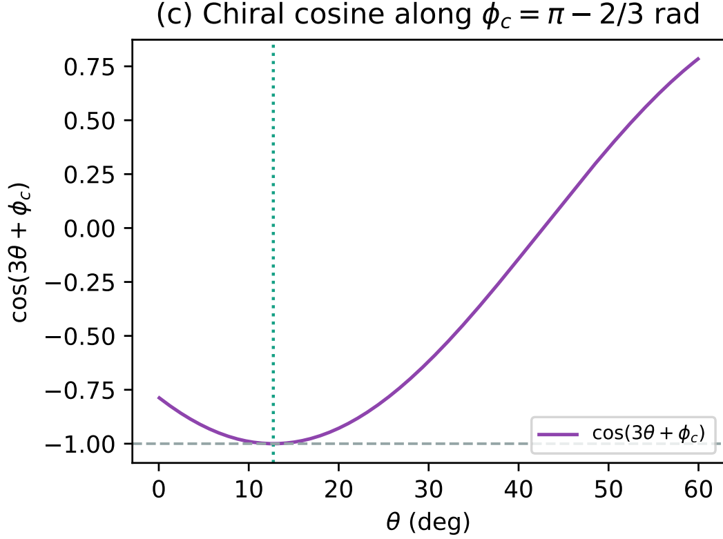
FIG. 2. The chiral cosine interaction evaluated along the derived vacuum phase \phi_c = \pi - 2/3 . The minimum rests cleanly at the predicted orientation \theta = 2/9 rad.
