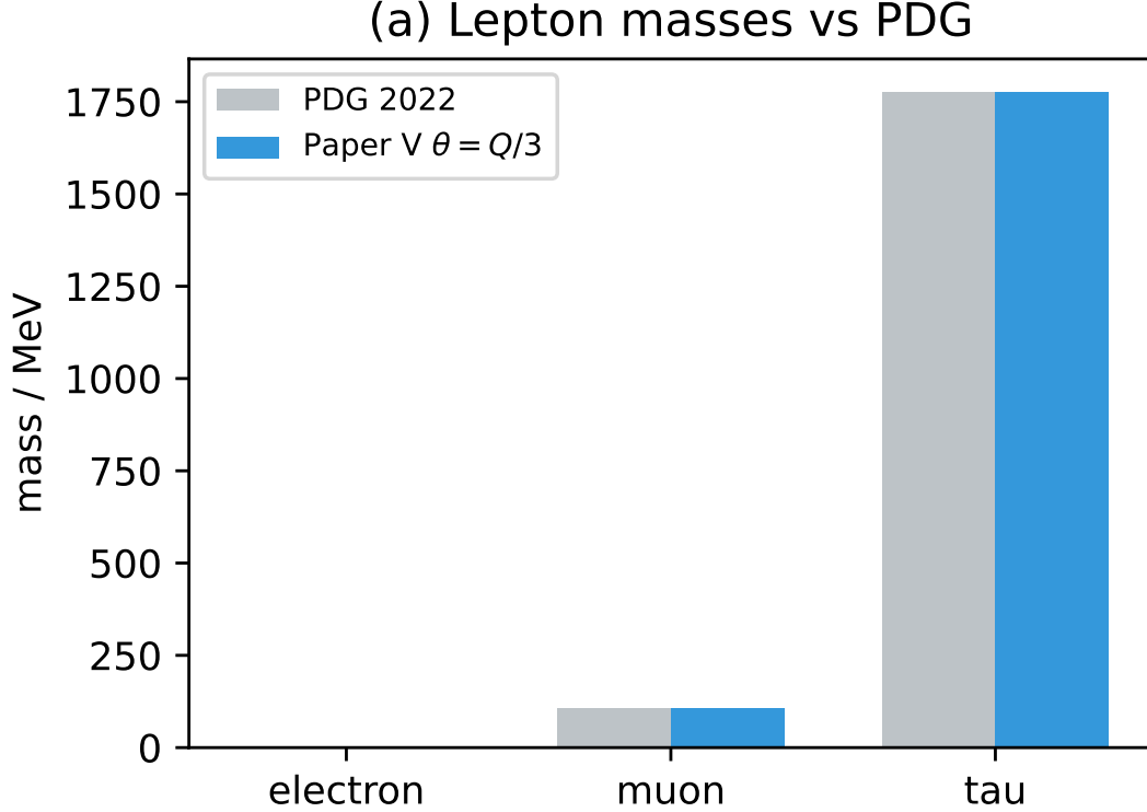
FIG. 3. Comparison of the lepton masses predicted by the zero-parameter CDFT derivation ( \theta = 2/9 rad) against the 2022 PDG measured values. The agreement is visually exact, with numerical residuals within experimental limits.
