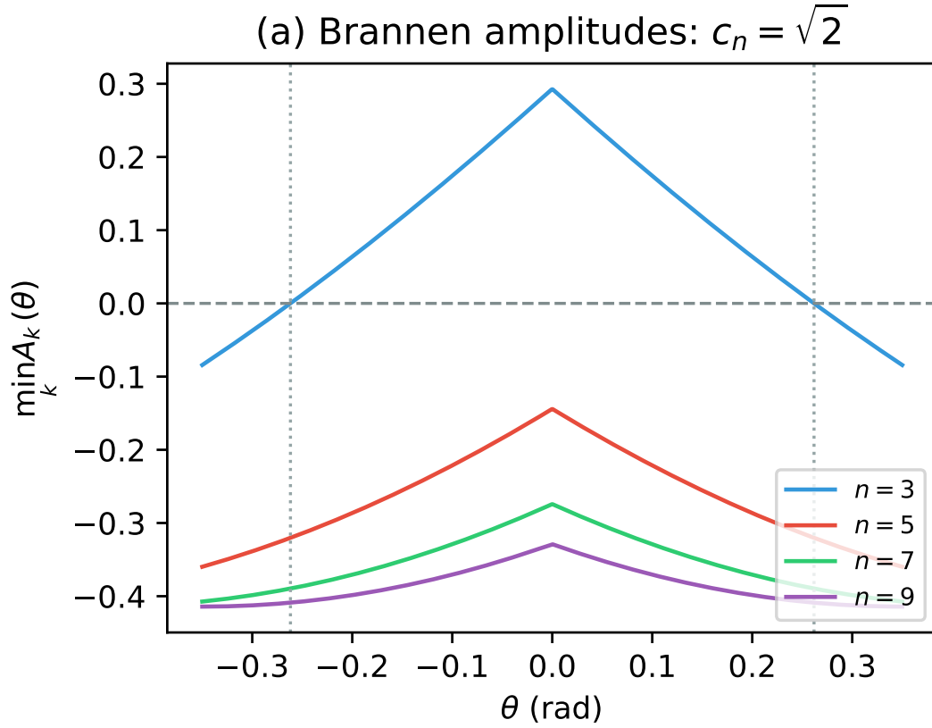
FIG. 1. Minimum amplitude over all modes as a function of the phase \theta . For n = 3 , there is a domain where all amplitudes are positive. For n \geq 5 , no such domain exists, obstructing the extension of the pure Koide formula.
