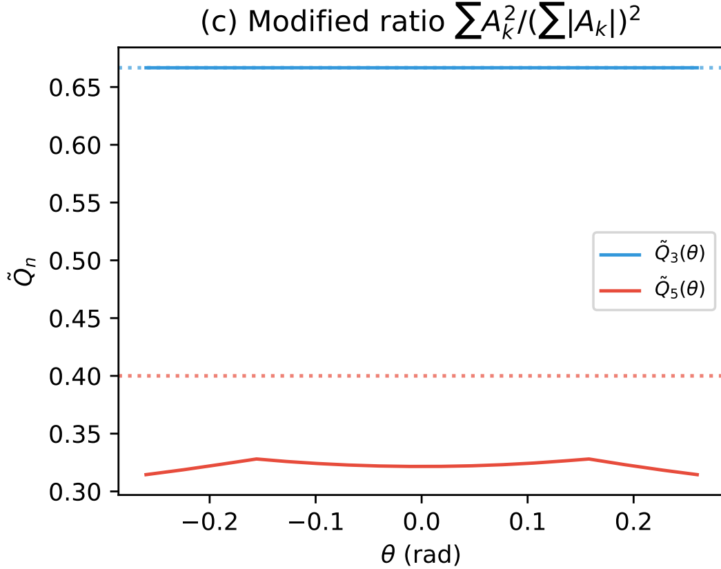
FIG. 3. The modified ratio \tilde{Q}_n(\theta) for n = 3 and n = 5 . While \tilde{Q}_3 is a strict constant ( 2/3 ), \tilde{Q}_5 varies and does not meet the 2/5 target.
