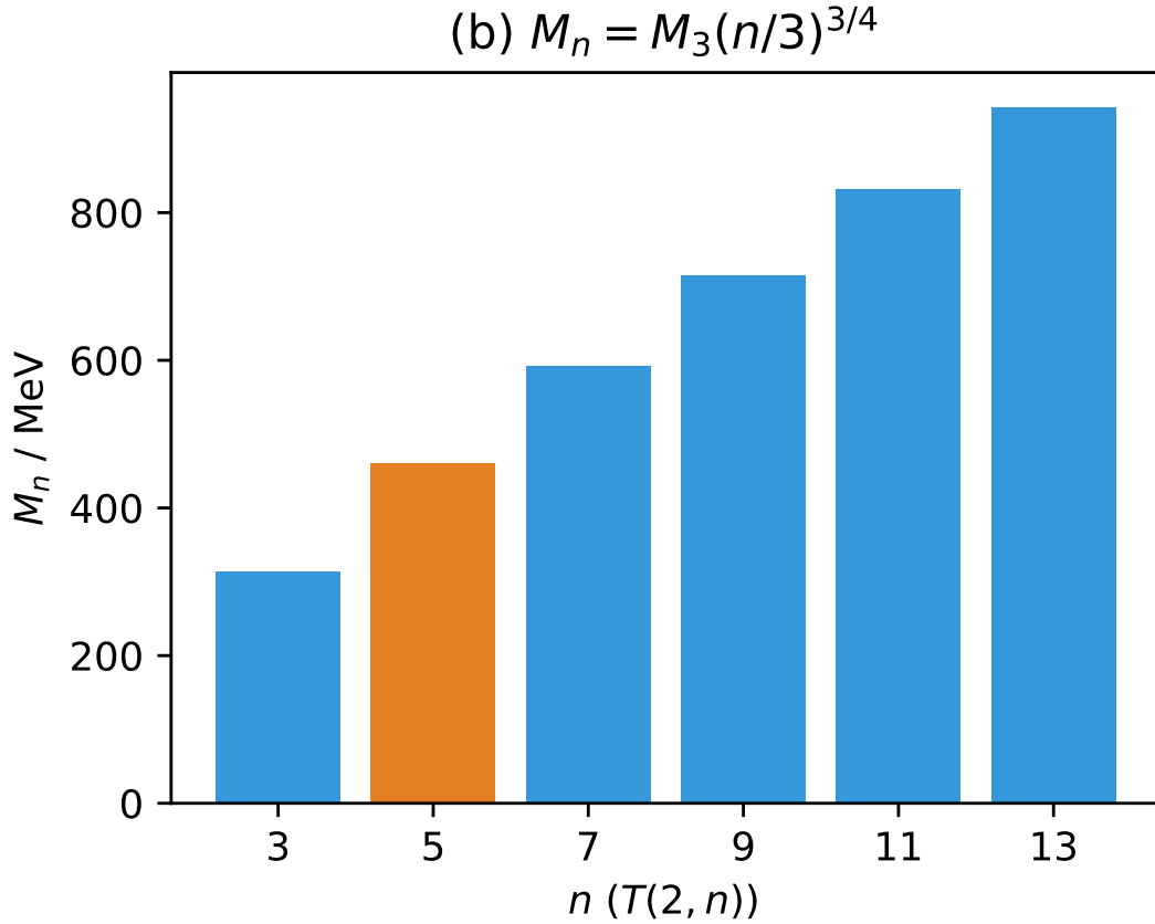
FIG. 2. The mass scales of the higher \mathbb{Z}_n knotted families, predicted by Faddeev-Niemi scaling directly from the lepton scale M_3 .
