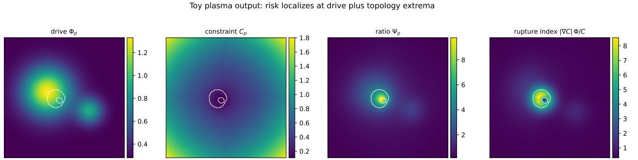
FIG. 4. Generated plasma output. The rupture index combines drive, constraint, and constraint-gradient information. In the toy field, risk does not follow the drive field alone. Summary table: table5_plasma_rupture_index_summary.csv .
