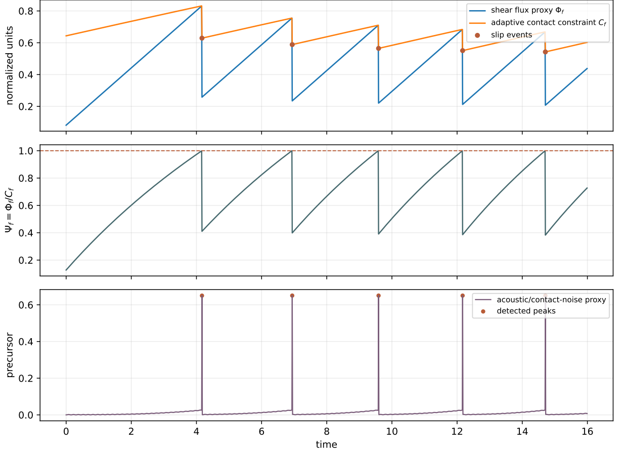
FIG. 2. Generated stick-slip output. A slowly increasing shear-flux proxy loads an adaptive contact constraint until release. The lower panel shows a precursor/noise proxy. Event table: table2_friction_stick_slip_events.csv .
