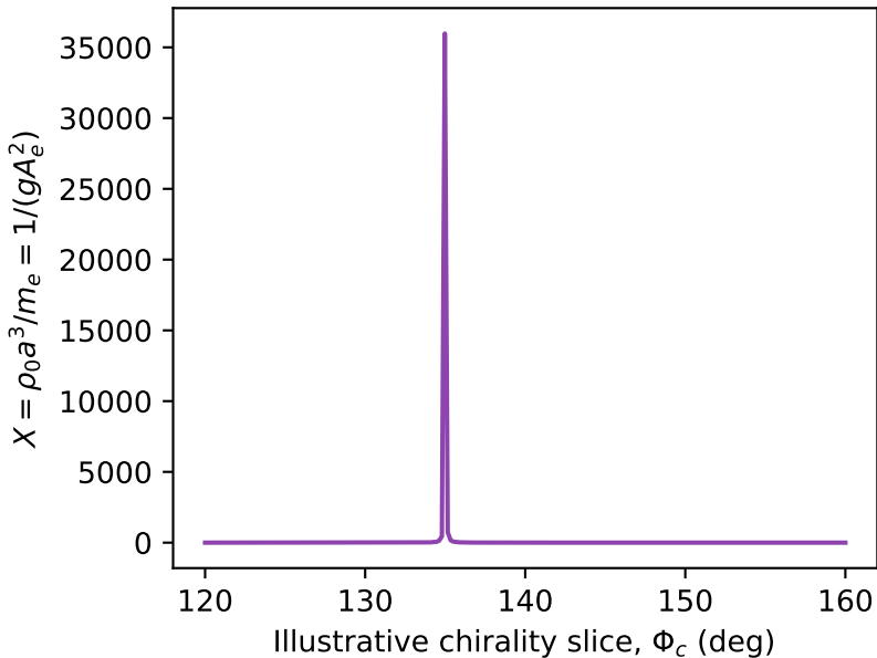
(b) Dimensionless coupling vs chirality slice
