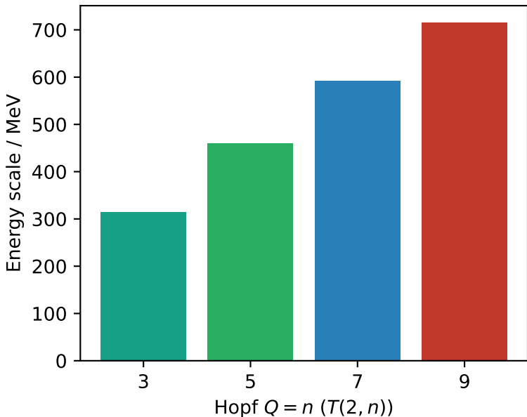
(c) Faddeev-Niemi family scaling from M_3
