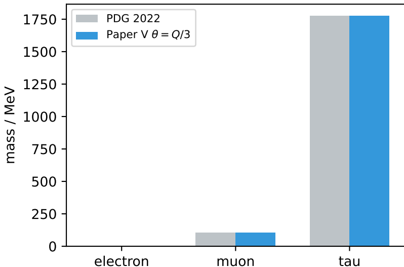
(a) Lepton masses vs PDG
