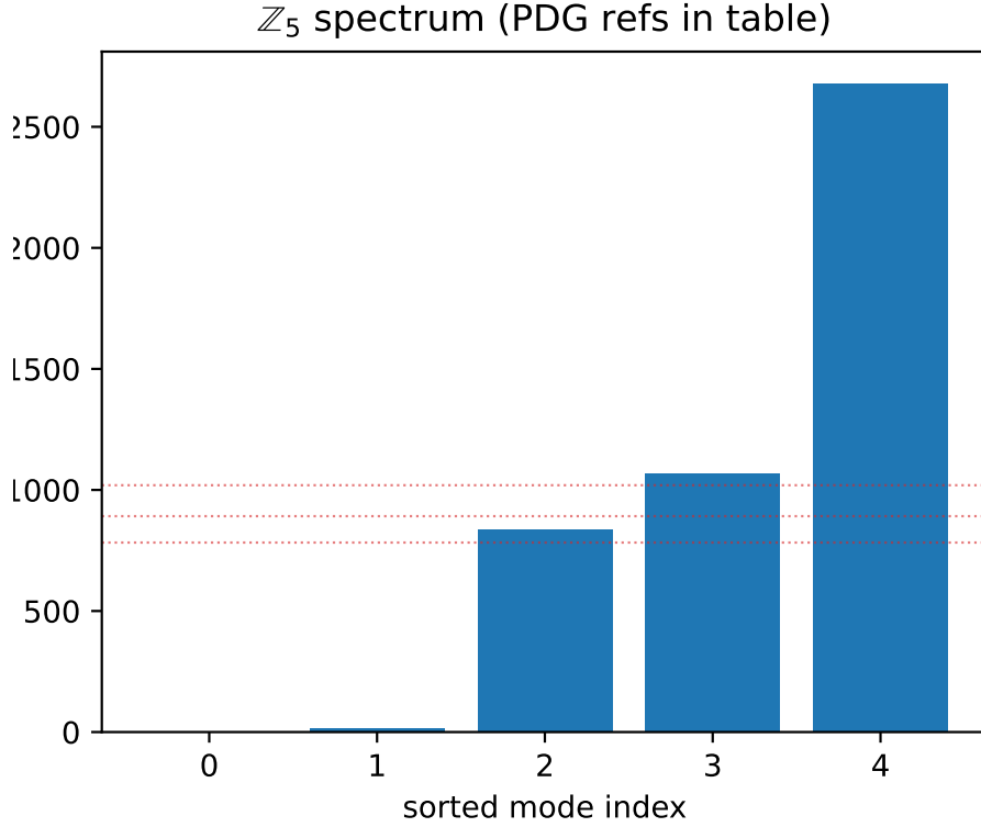
Figure 3: The \mathbb{Z}_5 cinquefoil mass spectrum. The three co-phase modes bracket the \omega , K^* , \phi , and f_0 light meson region.
