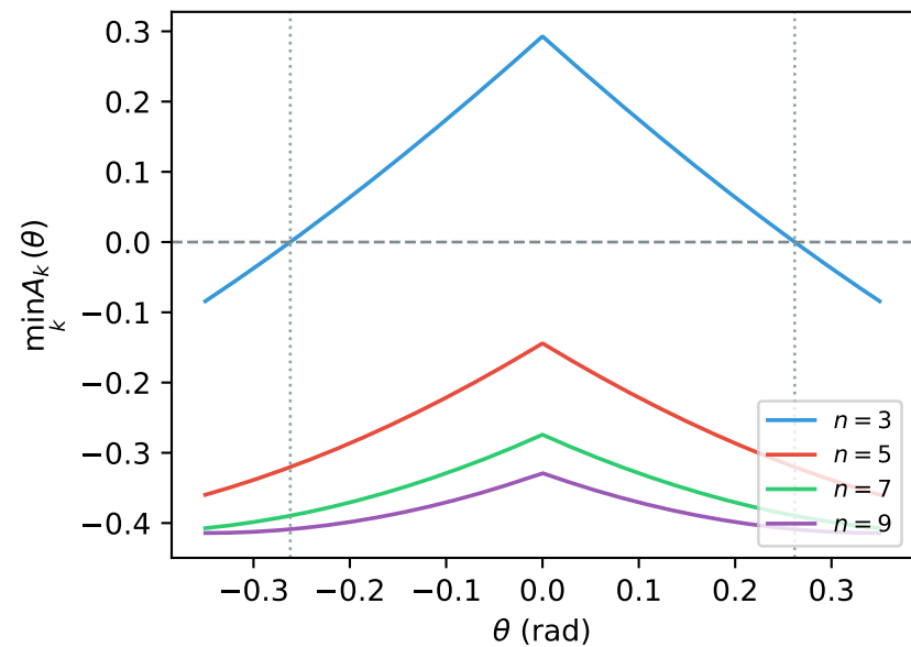
(a) Brannen amplitudes: c_n = \sqrt{2}
