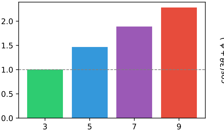
(a) Faddeev-Niemi scaling
