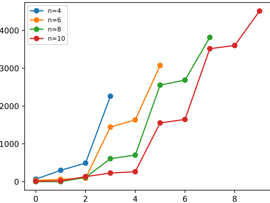
even-n spectra
