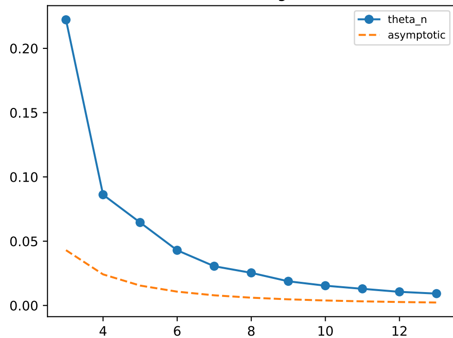
theta convergence
