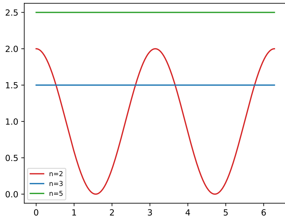
theta convergence
