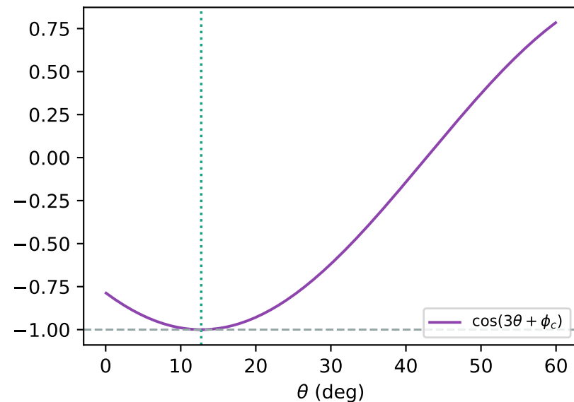
(c) Chiral cosine along \phi_c = \pi - 2/3 rad
