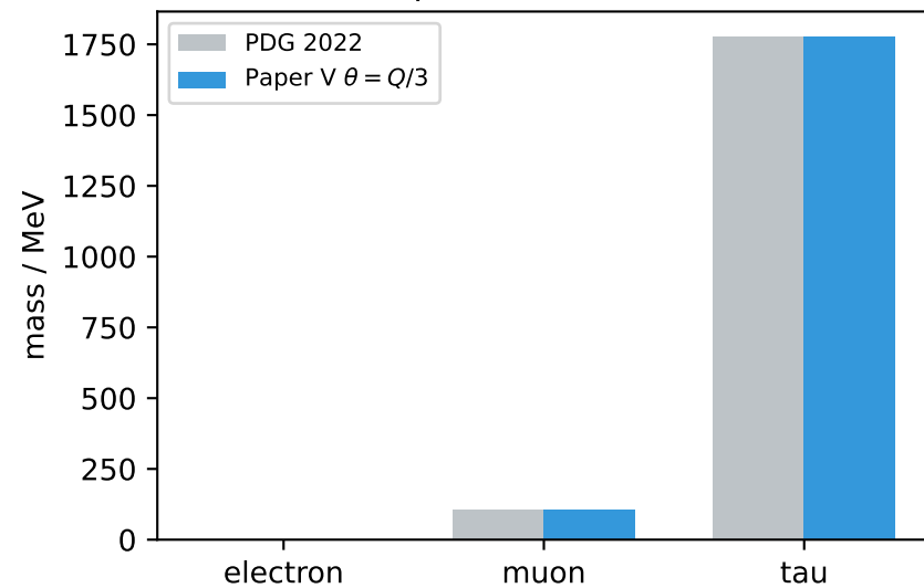
(a) Lepton masses vs PDG
